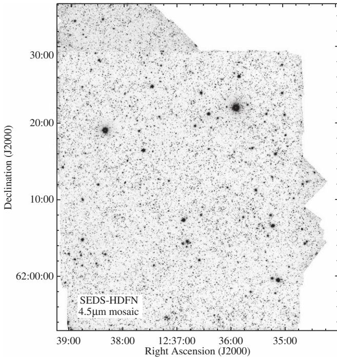
Figure 16. As Figure 15, but for the 4.5 \mu\text{m} mosaic.
