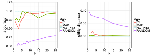
(a) Bank Dataset Accuracy (b) Bank Dataset Utility Distance Figure 11: Bank dataset result quality
