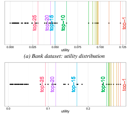
(a) Bank dataset: utility distribution (b) Diabetes dataset: utility distribution Figure 10: Distribution of Utilities
