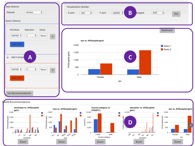
Figure 2: SEEDB Frontend
