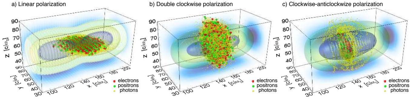
FIG. 1. 3D PIC simulation snapshot of QED cascades for a) Setup 1 with a_0 = 1000 at t = 90 \omega_0^{-1} , b) Setup 2 with a_0 = 1300 at t = 80 \omega_0^{-1} , c) Setup 3 with a_0 = 2000 at t = 46 \omega_0^{-1} . The laser pulses are shown through iso-contours of the electromagnetic energy. The particles displayed represent only a small fraction of the simulation particles.
