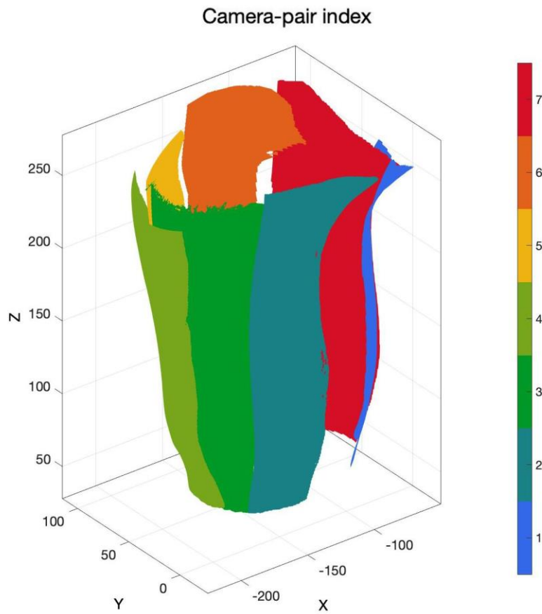
Figure 9: Image showing reconstructed 360° 3D geometry. While the surfaces do not perfectly align into the original shape, the numerical strain values are valid.
