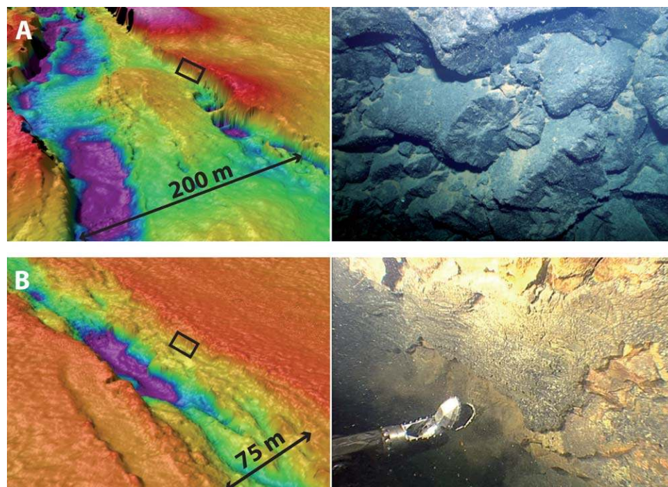
Figure 6. 3-D views (location on Figure 2) and photos (located by black rectangles) of a narrow (< 150 m wide) and a large (> 150 m) Axial Summit Trough (AST), showing the morphology of its bounding faults. (a) Border of a wide AST. The steep (> 70°) and sharp-edged fault exposes former pristine lava sections and is not covered by subsequent volcanic flows; (b) border of a narrow AST partially covered by lava deposits. The AST wall consequently displays a jagged shape, and nonuniform, moderate dips (< 55°). On the photo, the fault plane displays horizontal selvages reflecting the different lava lake levels during drainage. Photos acquired by the submersible Nautile during the PARISUB cruise (2010).
