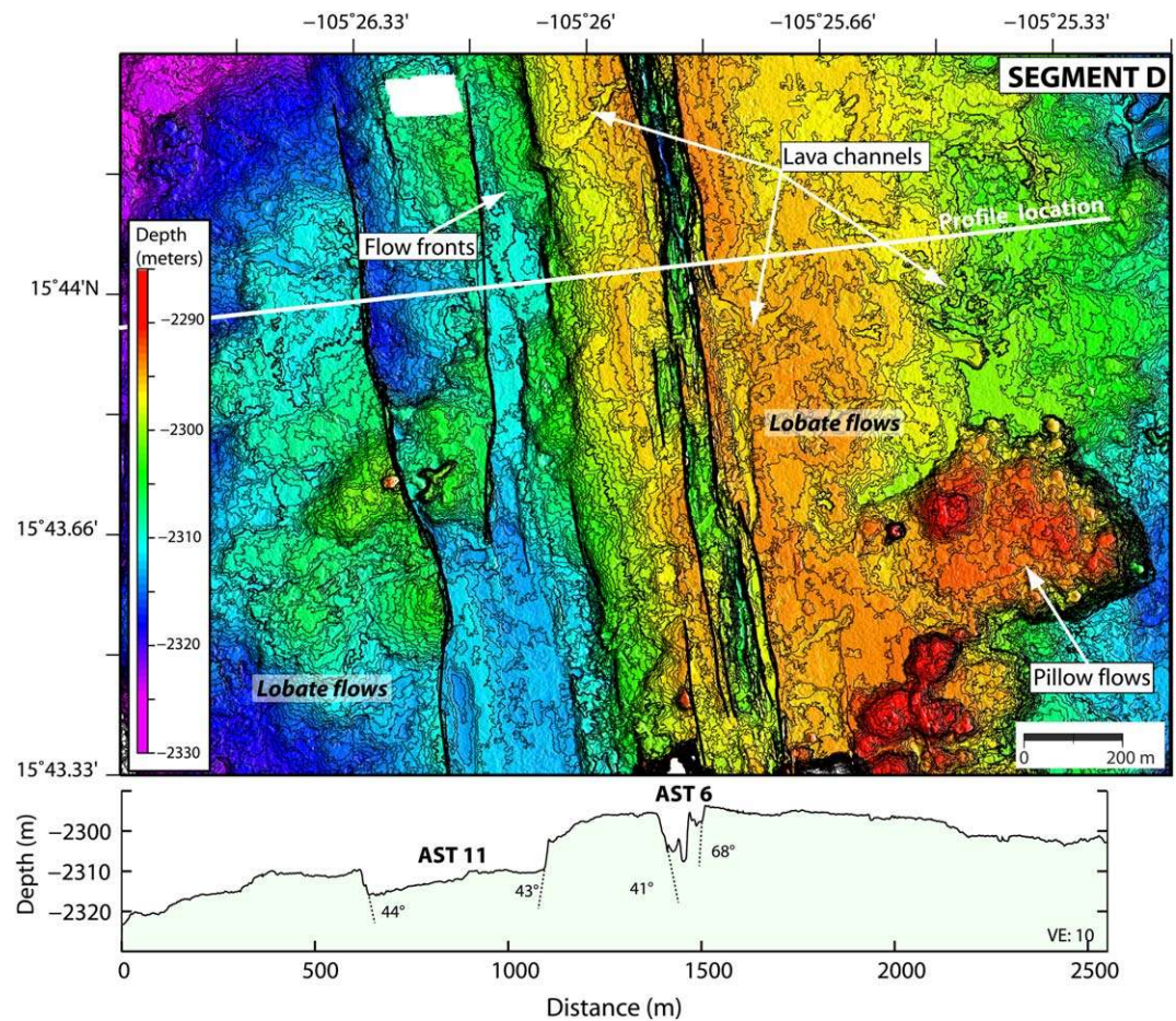
Figure 7. Detailed high-resolution (1 m grid cell size) bathymetry (see location on Figure 2) showing parallel Axial Summit Troughs AST 6 and AST 11 in the segment. The main lava flows morphologies and fault associated with ASTs (bold lines) are indicated. Lobate lava flows originating from AST 6 (which is centered on the axial dome) are transported both sides of the AST through lava channels. In the west, flows are clearly cut by the AST 11, which is itself partially filled with more recent lobate lava emitted from the eastern AST 6. The bathymetric profile highlights the differences in the geometry of the two contiguous ASTs.
