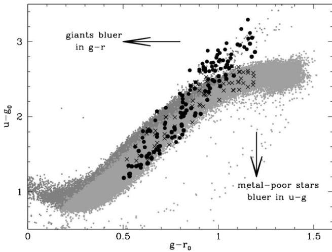
Figure 10. Red giant selection—a demonstration of how the K giant locus crosses from the blue ( u - g ) side of the stellar locus at g - r = 0.6 over to the red side of the locus at g - r = 1.0 . M giants with TiO features appear at g - r > 1.3 and u - g > 3.0 . The small dot shows the photometric stellar locus in a SEGUE high-latitude field (there are Sagittarius M giants present at the end of the locus). Stars with l -color greater than 0.07 are shown in light gray. Spectroscopically confirmed dwarfs are shown with large crosses, giants with large filled circles.
