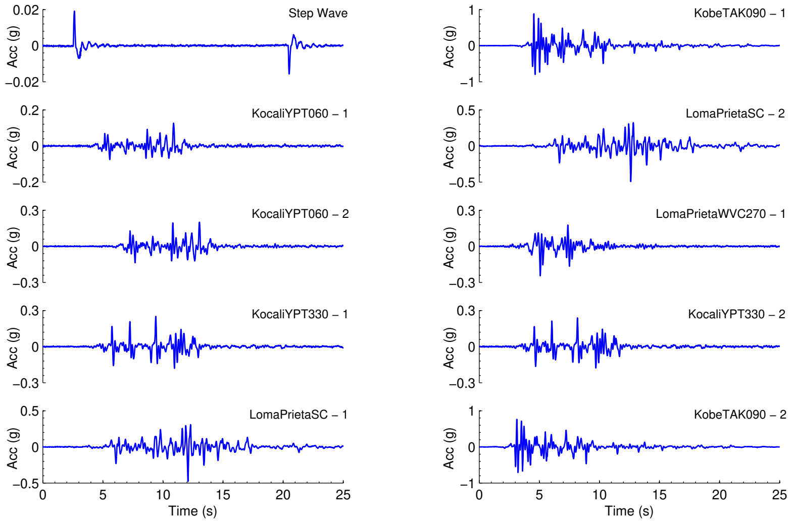
Figure 3.15 History of input acceleration in model GC01.
