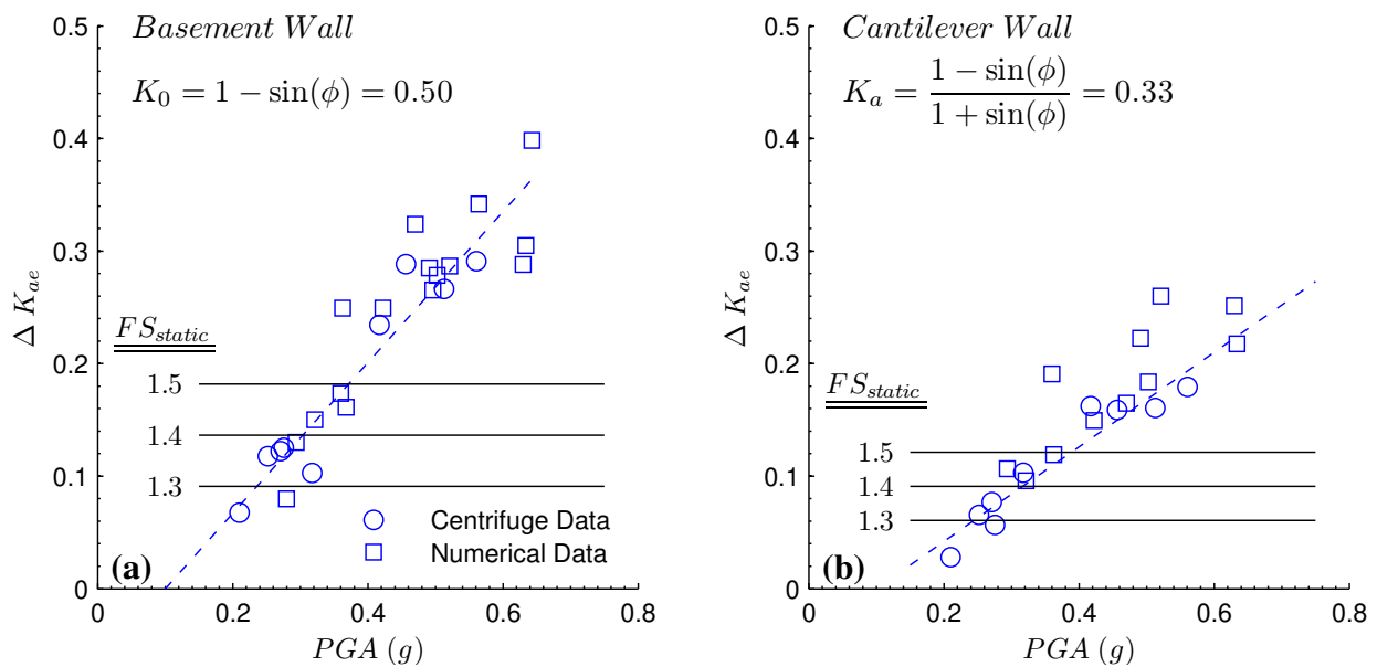
Figure 8.6 Seismic load increments in the basement and cantilever walls. Load increments below the FS_{static} lines need not be included in the wall design.
