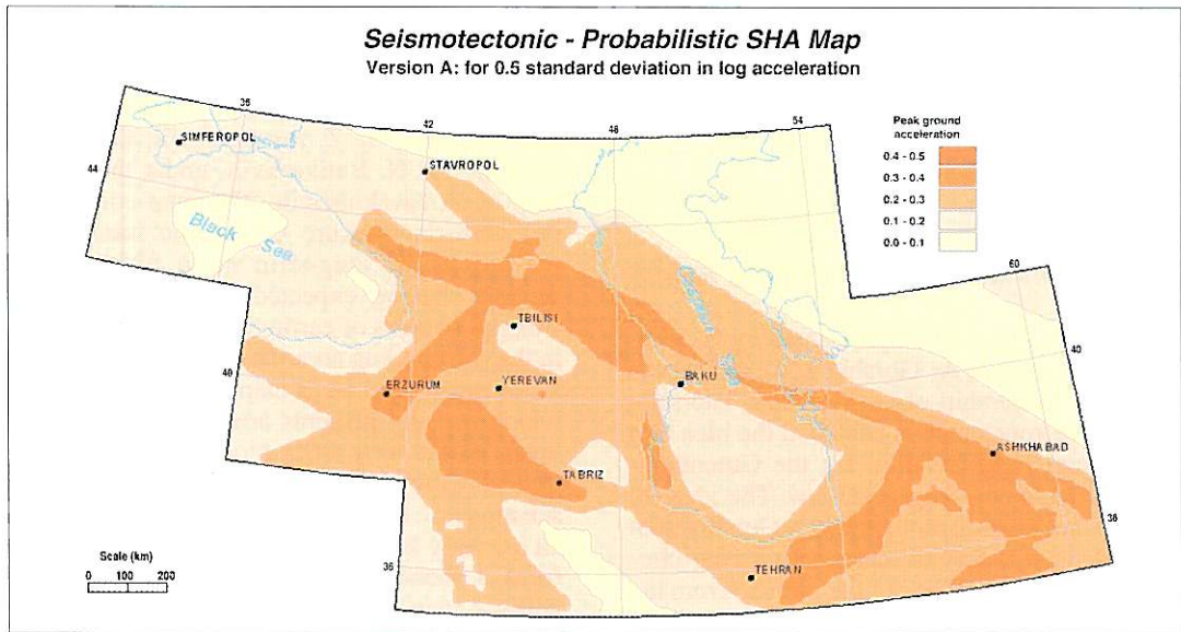
Fig. 5. Seismic hazard map of the Caucasus test area computed using the seismotectonic probabilistic approach and adopting a 0.5 standard deviation to characterize the attenuation uncertainty. Peak ground acceleration expected with a 10% exceedance probability in 50 years (return period of 475 years) is displayed.
