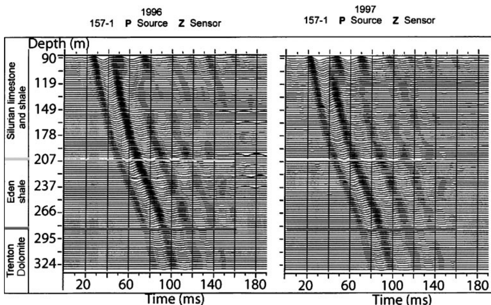
Figure 11. Downgoing wavefields for 1996 (left) and 1997 (right) show no visible changes, except a constant time shift associated with near-surface effects.
