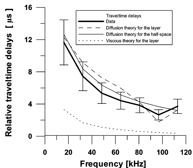
Figure 6. Travelt ime delays of a reflected wave from a dry layer with respect to a water-saturated layer. Data curve (thick solid line) is compared with the theoretical diffusive-viscous model (dashed line) and purely viscous model (dotted line). A theoretical curve for a diffusive-viscous half-space is shown as thin solid line.
