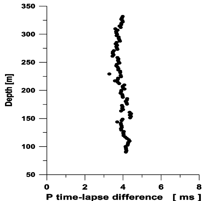
Figure 8. Time-lapse change for the NIPSCO VSP P-wave data from site 1 (a 30-m offset). We show the difference in P-wave arrival time, at each recorded depth, between the 1996 (gas-saturated reservoir) and 1997 (water-saturated reservoir) data. No change was observed in the reservoir horizon (~300–310 m) compared with the other horizons, within the scatter in the data.
