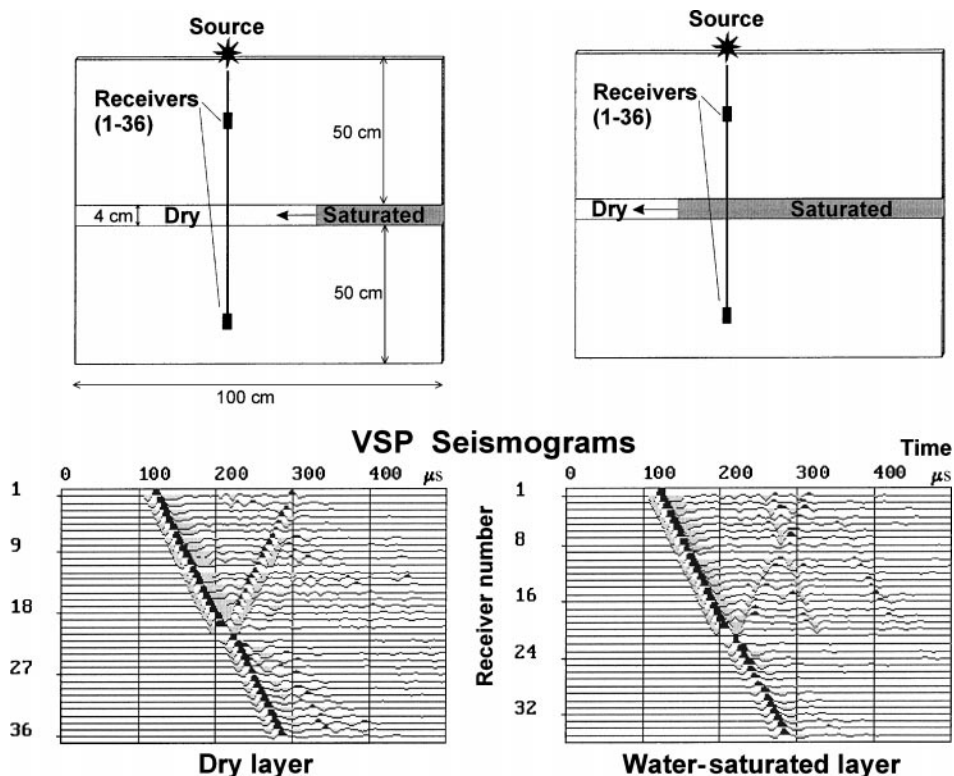
Figure 2. Physical modeling experimental setup (upper panels) and recorded traces (lower panels) for porous-layer attenuation measurements in dry (left) and water-saturated (right) layers.
