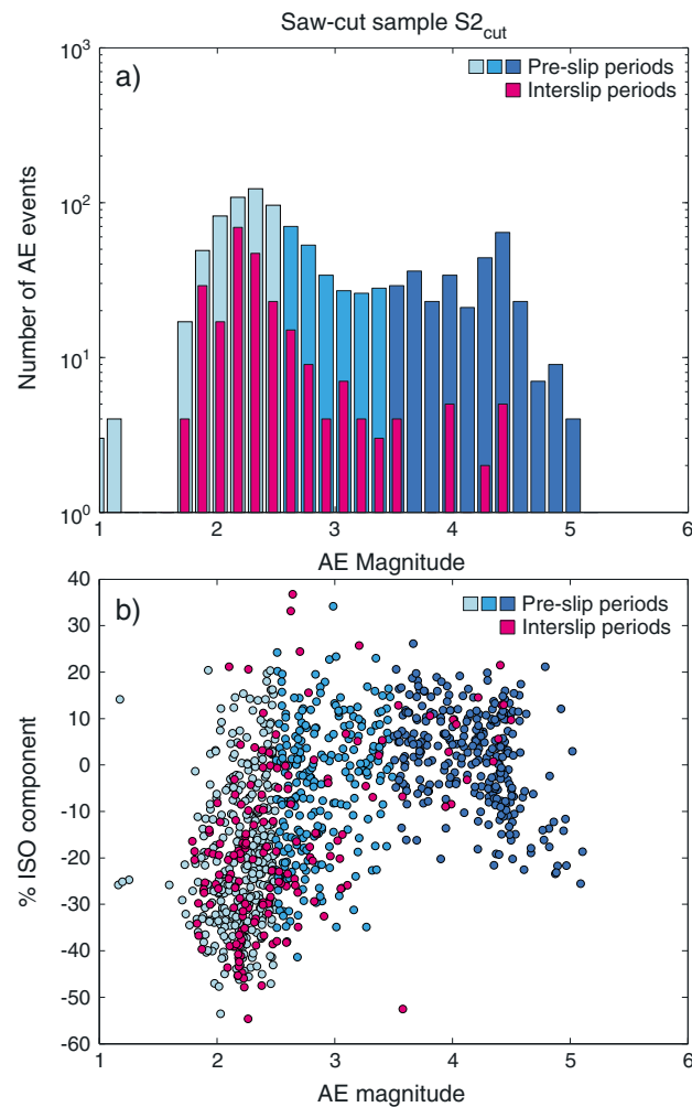
Figure 3. (a) Comparison of FMDs computed for AEs occurring during preslip and interslip periods of experiment S2 cut . (b) Relationship between AE magnitude and the amount of ISO component for AEs from preslip and interslip periods. Note that the AE magnitude is specific to the here employed transducers and is not calibrated in an absolute sense.
