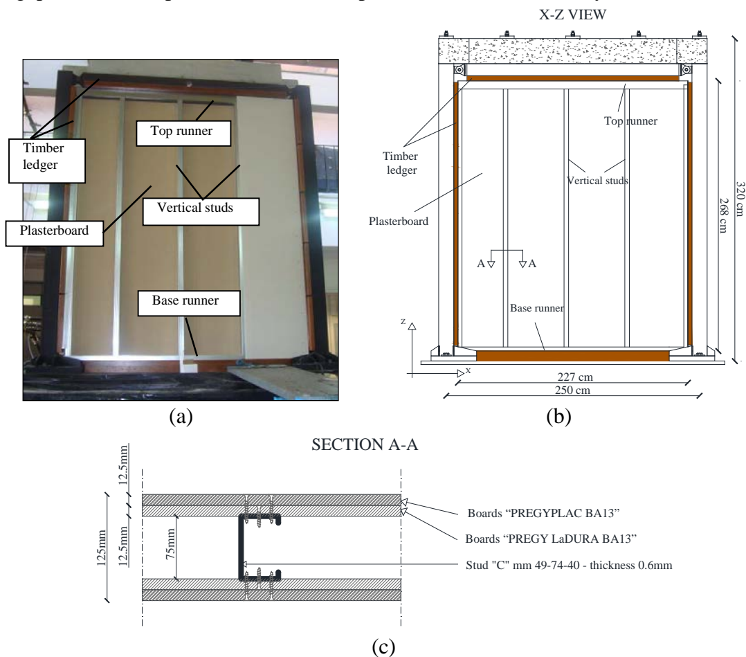
Fig. 2 Internal plasterboard partition: (a) overview; (b) graphical scheme; (c) horizontal cross section
