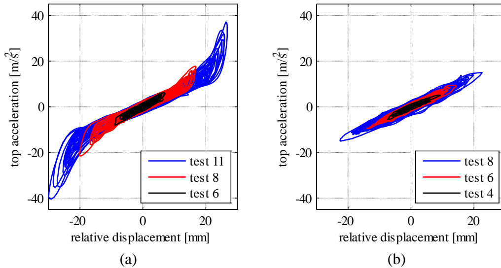
Fig. 9 Top acceleration vs relative displacement plot for the different seismic tests in (a) X direction (b) Y direction
