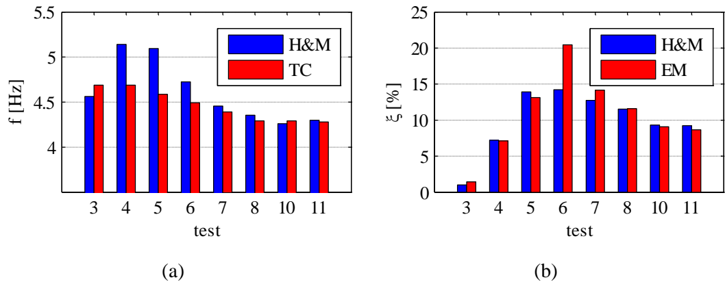
Fig. 10 (a) Natural frequency evaluation according to Hashemi and Mosalam (2006) (H&M) procedure and transfer curve method (TC) for the different seismic tests; (b) damping ratio evaluation according to Hashemi and Mosalam (2006) (H&M) procedure and the energetic method (EM) for the different seismic tests
