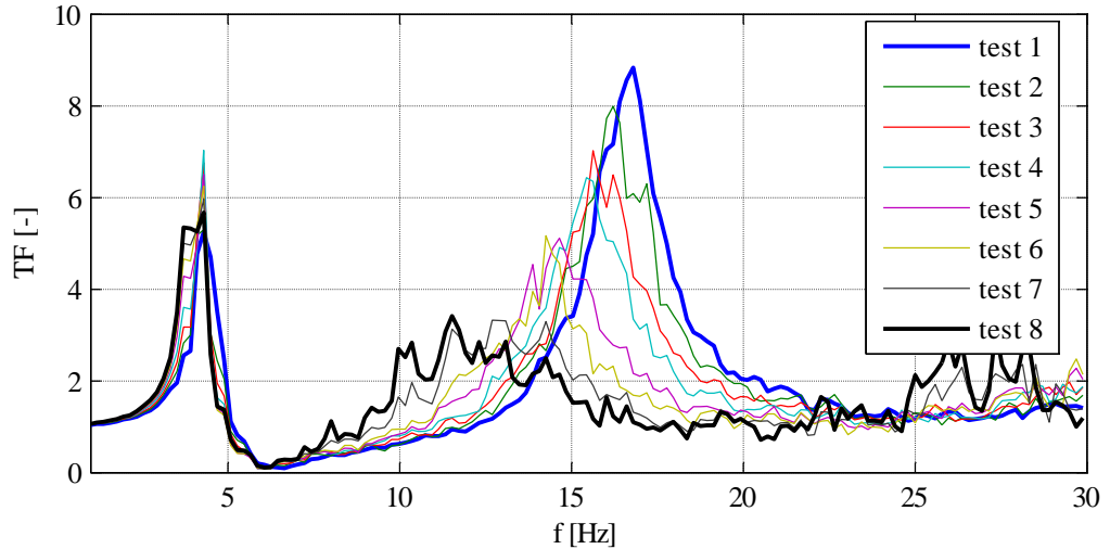
Fig. 12 Transfer function from the base to the partition centre in the out of plane direction for the bidirectional tests
