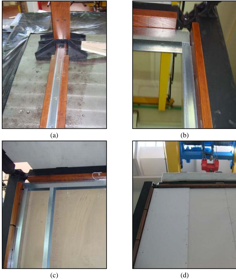
Fig. 5 Installation procedure: (a) base runner; (b) top and lateral runners; (c) vertical studs; (d) plasterboard second (outer) layer
