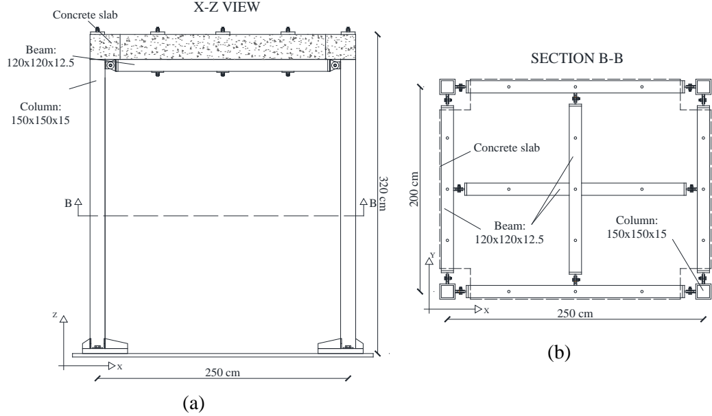
Fig. 3 Scheme of test setup: (a) lateral view, (b) horizontal cross section
