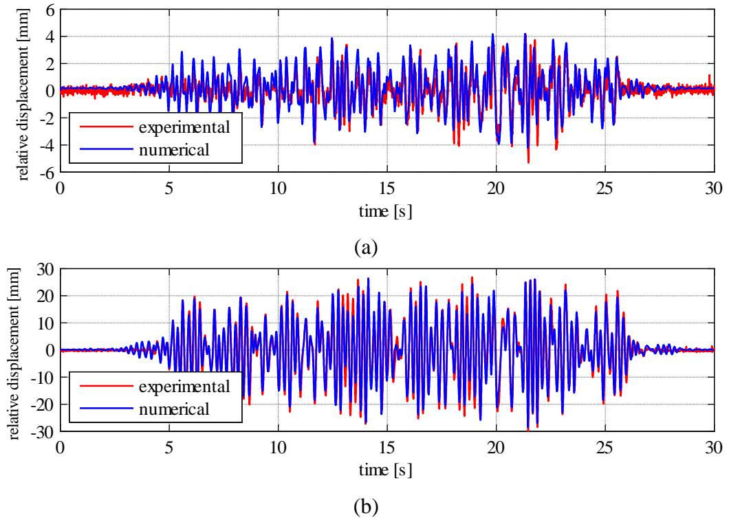
Fig. 14 Comparison between experimental and numerical time histories: (a) test 6; (b) test 11
