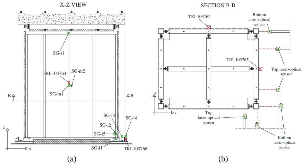
Fig. 6 Scheme of test instrumentation: (a) lateral view; (b) horizontal cross section
