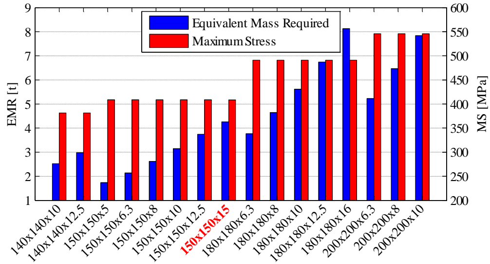
Fig. 4 Parametric study for the definition of the column cross sections: Equivalent Mass Required (EMR) and the Maximum Stress (MS) for each considered column cross section
