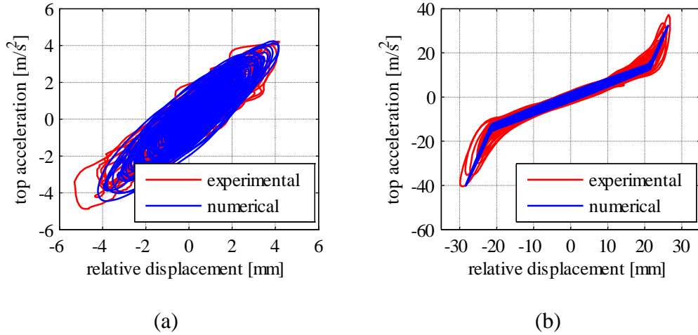
Fig. 13 Comparison between experimental and numerical hysteresis loop: (a) test 6; (b) test 11
