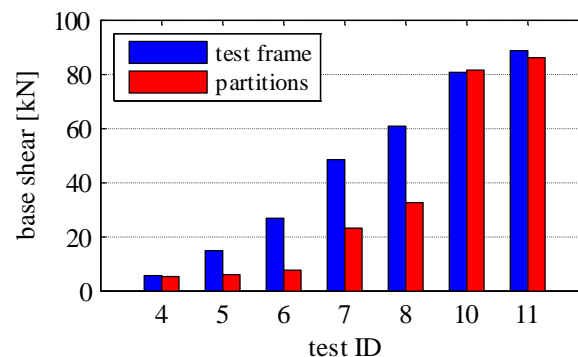
Fig. 11 Base shear repartition between test frame and partition systems for the different seismic tests
