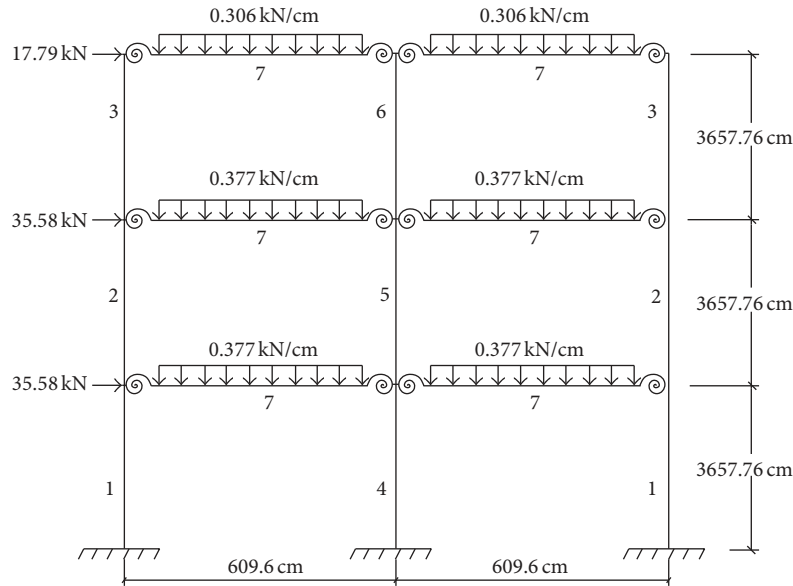
FIGURE 4: Unbraced steel portal frame with semirigid connections [21].
