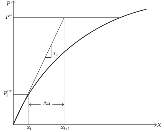
FIGURE 3: Newton-Raphson solution, one iteration.
