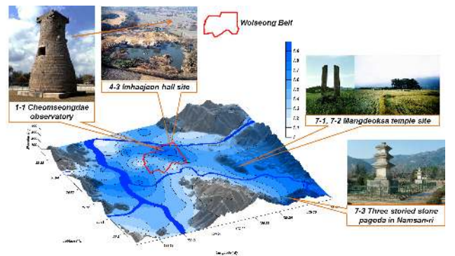
Fig. 9. GIS based geotechnical information system for peak ground surface acceleration for the earthquake level of 1000 yr return period and the cultural heritage areas which have relatively high potentials for site amplification.
