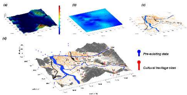
Fig. 7. The procedure of seismic microzonation: (a) three-dimensional digital elevation map by the triangulated irregular network; (b) kriging interpolation of geotechnical value; (c) standard geographical information map; (d) combination of digital maps.
