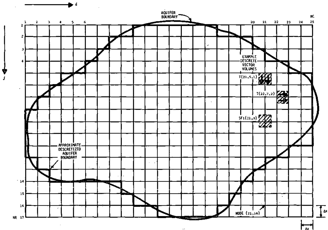
Figure 7. Plan view of finite difference grid over map of aquifer system
