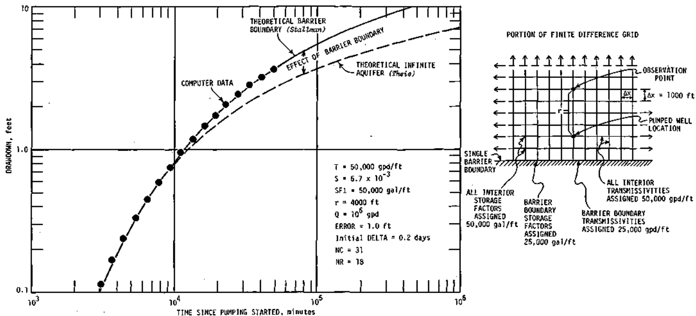
Figure 21. Comparison of theoretical and digital computer solutions for barrier boundary conditions
