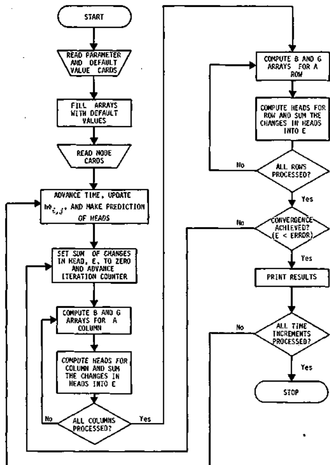
Figure 10. Flow chart for basic aquifer simulation program
