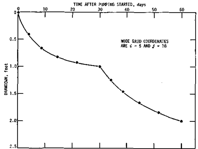
Figure 69. Time-drawdown curve for sample problem
