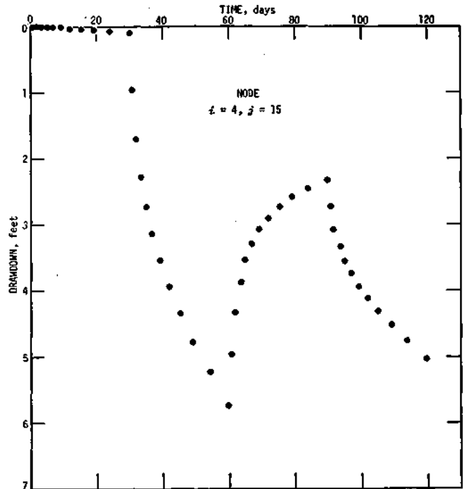
Figure 34. Example time-drawdown graph for variable pumping scheme
