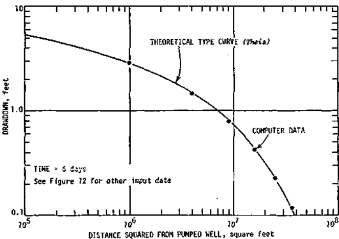
Figure 15. Distance-drawdown comparison of theoretical and digital computer solutions
