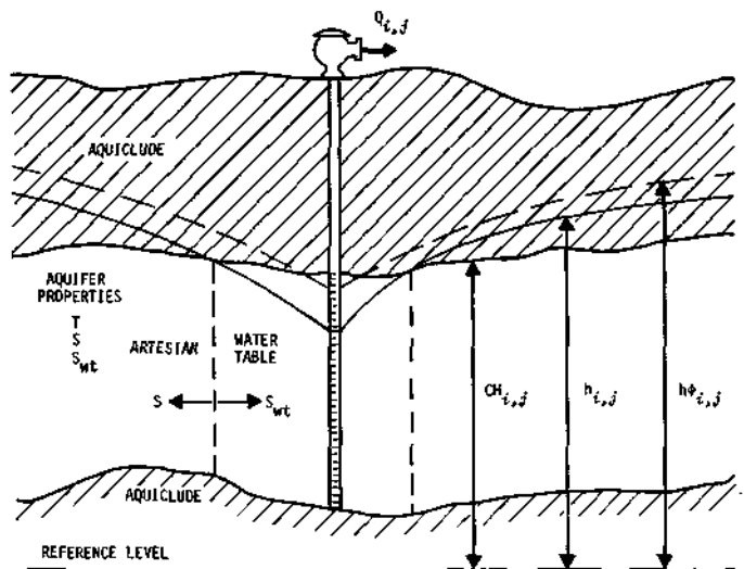
Figure 54. Basic aquifer simulation program parameters with storage coefficient conversion conditions
