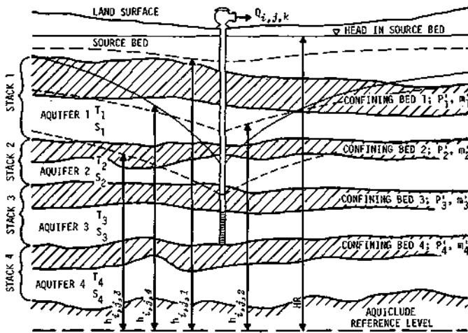
Figure 64. Aquifer simulation program parameters in three dimensions
