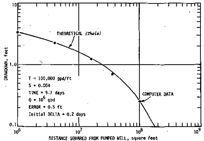
Figure 25. Distance-drawdown comparison of theoretical and computer solutions with data from variable grid spacing model
