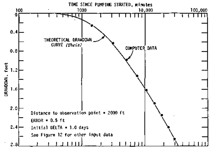
Figure 18. Comparison of theoretical and digital computer solutions using nonuniform time increments
