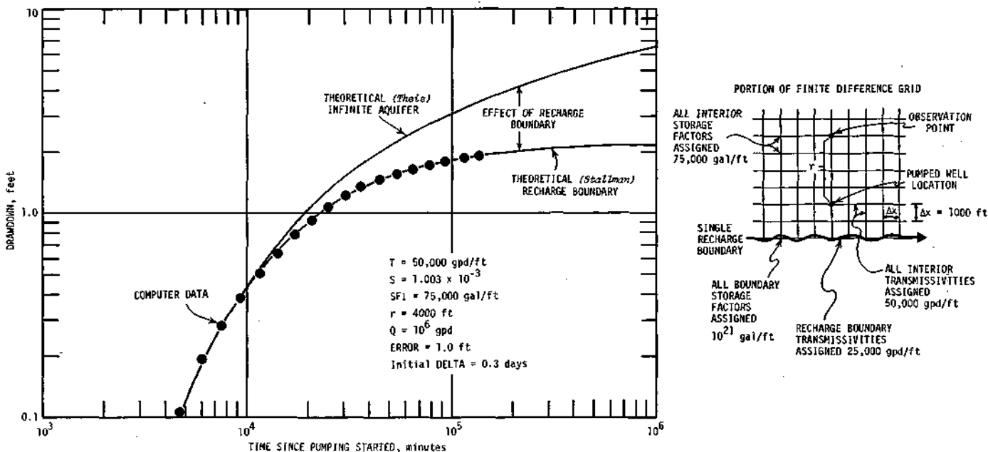
Figure 22. Comparison of theoretical and digital computer solutions for recharge boundary conditions
