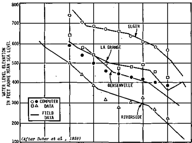
Figure 77. Comparison of actual and digital model declines in piezometric surface of Cambrian-Ordovician aquifer 1864-1958
