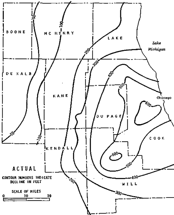
Figure 77. Comparison of actual and digital model declines in piezometric surface of Cambrian-Ordovician aquifer 1864-1958
