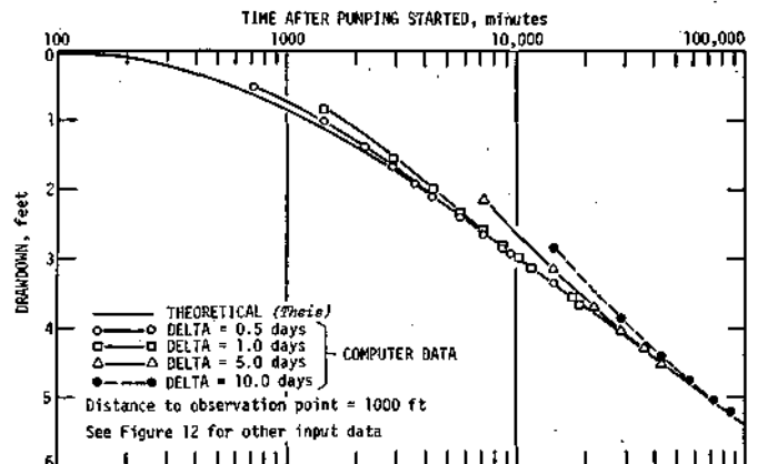
Figure 13. Comparison of theoretical and digital computer solutions near a pumped well with DELTA as a variable
