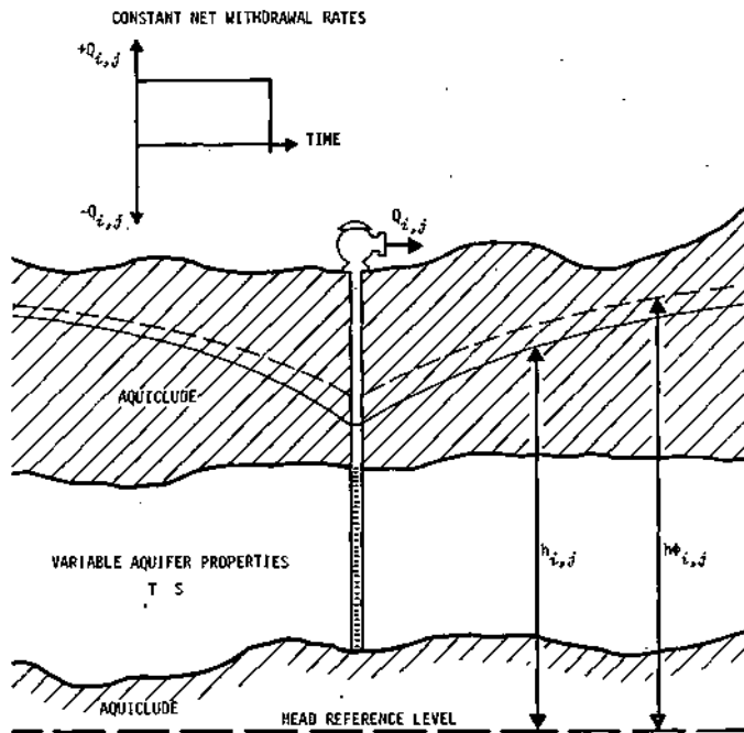
Figure 6. Generalized aquifer cross section for basic aquifer simulation program parameters
