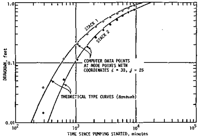
Figure 65. Comparisons of theoretical and computer simulated curves for three-dimensional problem
