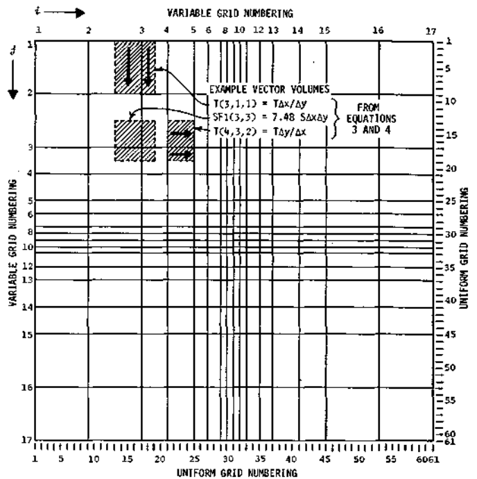
Figure 24. Example variable grid spacing model
