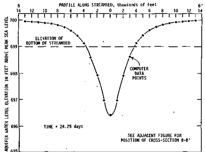
Figure 46. Head distribution in aquifer beneath streambed for induced infiltration problem
