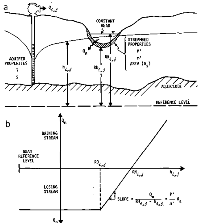
Figure 42. Basic aquifer simulation program parameters with induced infiltration (a) and head-infiltration rate curve (b)
