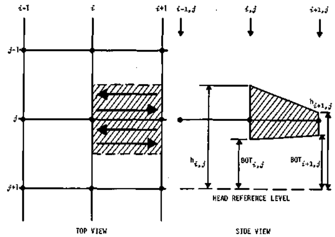
Figure 61. Typical vector volume of aquifer model for water table conditions
