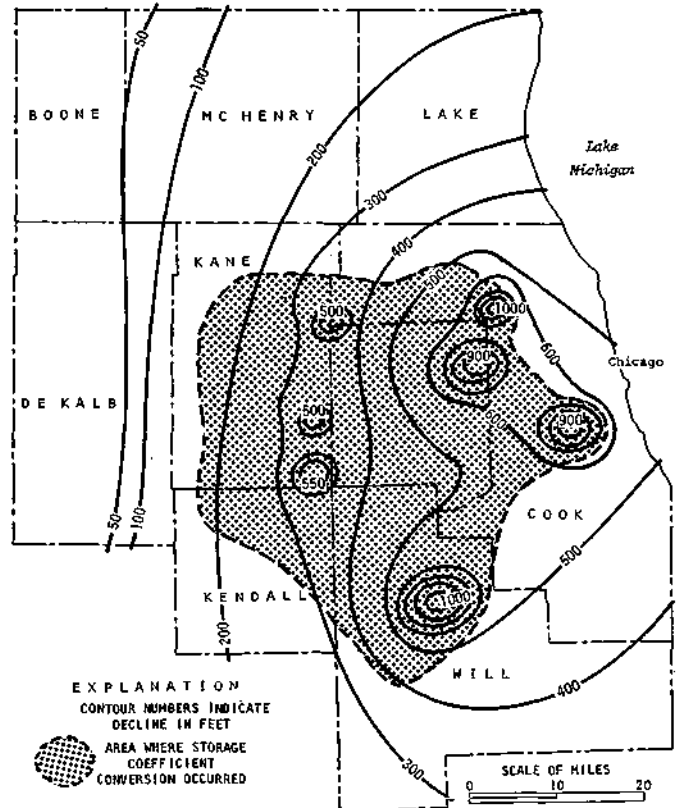
Figure 79. Model computed declines in piezometric surface of Cambrian-Ordovician aquifer 1864-1995
