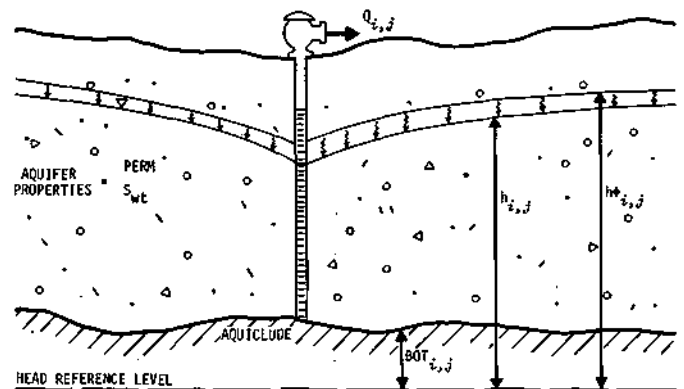
Figure 59. Basic aquifer simulation program parameters with water table conditions
