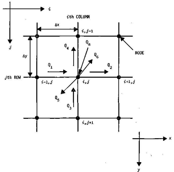
Figure 1. Finite difference grid
