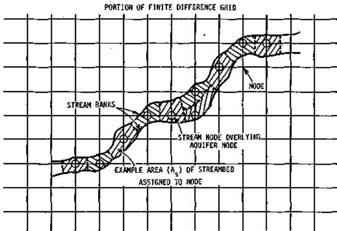
Figure 43. Example streambed vector volumes
