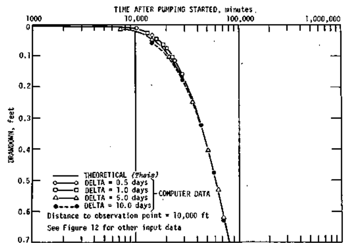
Figure 14. Comparison of theoretical and digital computer solutions distant from a pumped well with DELTA as a variable
