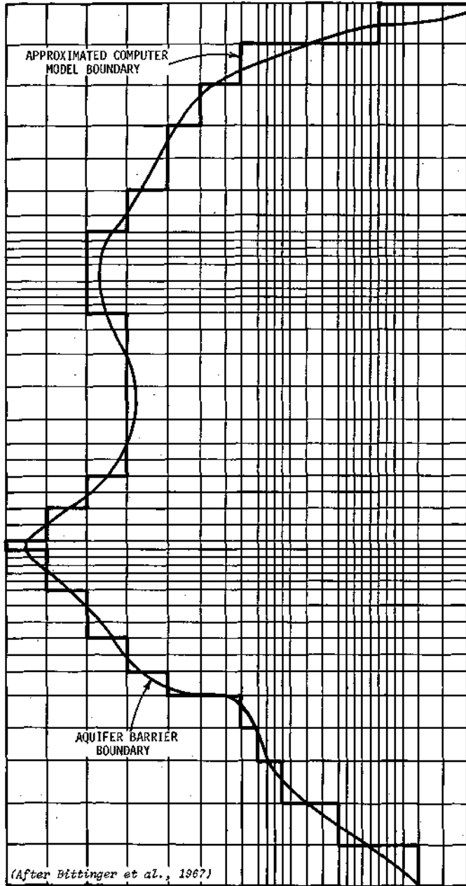
Figure 23. Finite difference grid using variable spacing
