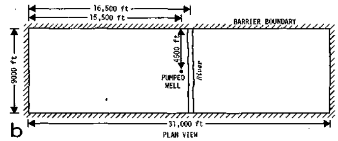
Figure 70. Example problem for combined aquifer simulation program
