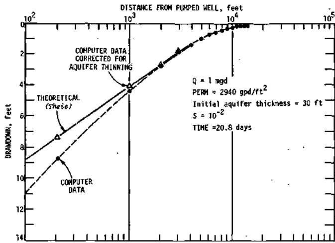
Figure 60. Comparison of computed and theoretical distance-drawdown curves for water table conditions
