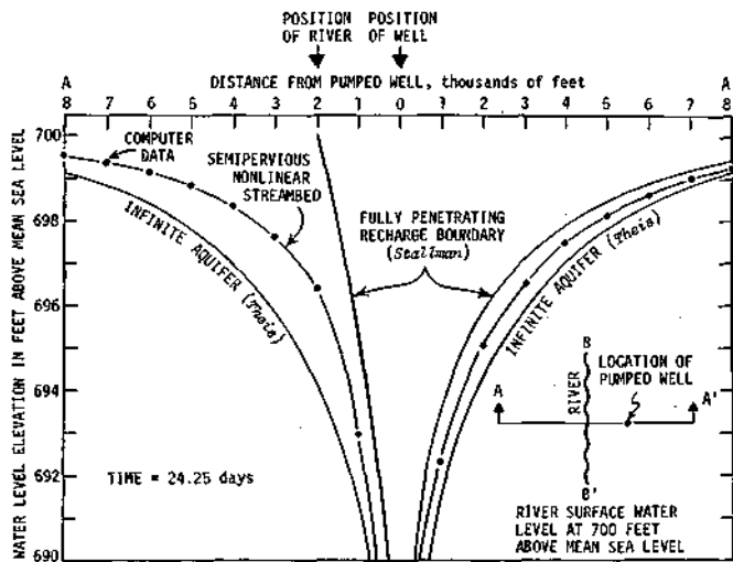
Figure 45. Cross section distance-drawdown graphs for induced infiltration problem
