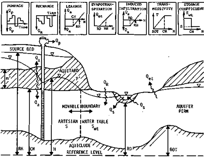
Figure 68. Combined aquifer simulation program parameters
