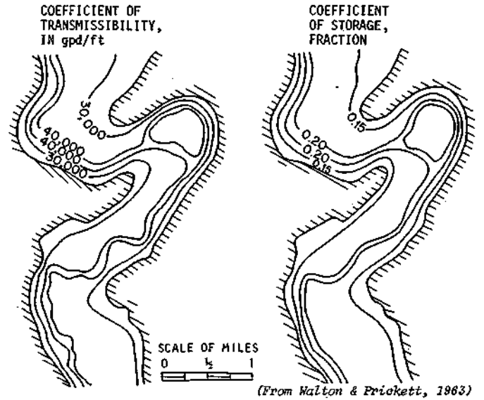
Figure 81. Diagrams of complex aquifer situation
