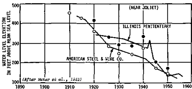
Figure 78. Decline of artesian pressure in selected deep wells in Chicago region
