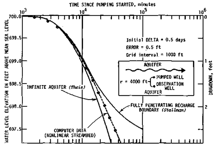
Figure 44. Time-drawdown curves for induced infiltration problem
