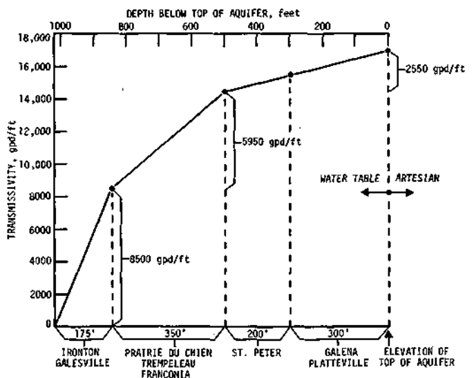
Figure 73. Transmissivity variation of units of Cambrian-Ordovician aquifer in Chicago region
