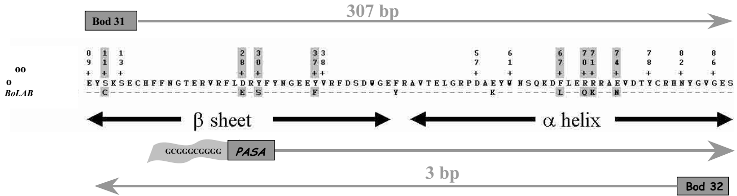
Figure 1. Amino acid residues constituting the CESFLQKN susceptibility marker in exon 2 of the BoLA-DRB3*09 allele.
