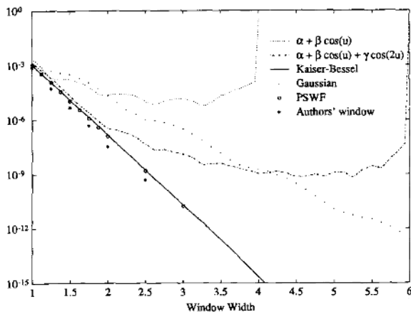
Fig. 5. A comparison of several convolving functions of varying widths, showing the relative amount of unwanted sidelobe energy that will alias into the center region of an image. This center region contains the entire region of interest if the sampled data was gridded onto a 2 \times subsampled grid.
