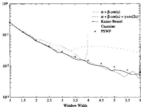
Fig. 3. A comparison of several convolving functions of varying widths, showing the relative amount of unwanted sidelobe energy that will alias into the image if that convolving function is used in the gridding algorithm. Note that when the two-term cosine function reaches a width of four, or when the three-term cosine function reaches a width of six, the first sidelobe of the function's inverse Fourier transform occurs within the image.
