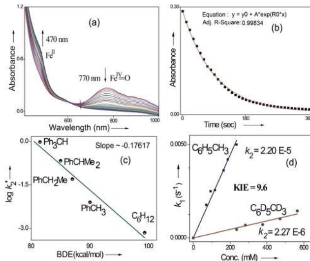
Fig. 4 (a) UV-vis change during C–H oxidation of ethylbenzene, (b) time trace of 2 at 770 nm, (c) bond dissociation energy (BDE) correlation plot: Bell–Evans–Polayni plot during C–H oxidation by 2 and (d) kinetic isotope effect study (kinetic studies were carried out under a N_2 atmosphere at 25 °C).
