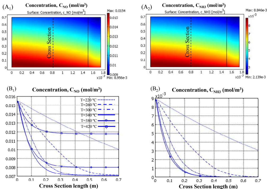
Figure 12: Variation of NO and \text{NH}_3 concentrations along the honeycomb reactor, C_{\text{NO}_{\text{in}}} = 350 ppm, C_{\text{NH}_3_{\text{in}}} = 200 ppm, GHSV=15000, other conditions: see Figure 9.
