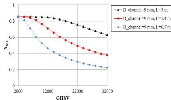
Figure 17: Effect of reactor channel length on NO conversion in the honeycomb reactor, T=300 °C, d_{\text{chan}}=9 mm, d_{\text{cat}}=0.5 mm, other conditions: see Figure 9.
