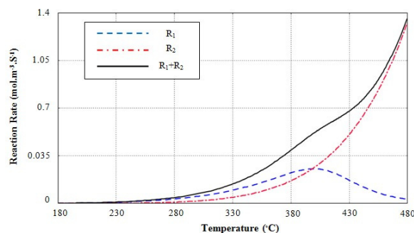
Figure 6: Calculated values of reaction rates R 1 and R 2 for inlet concentration values, conditions: see Figure 5.
