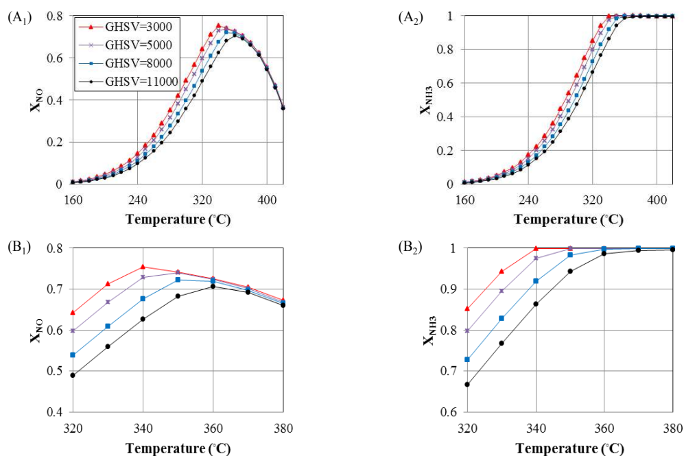
Figure 8: Evaluation of the effect of GHSV on conversion versus the gas temperature in the catalytic filter, C_{NO\_in}=C_{NH_3\_in}=350 ppm, C_{O_2\_in}=7.6 vol.%, \epsilon_p=0.95 , k=10^{-8} m 2 , d_{chan}=0.015 mm, d_{cat}=0.001 mm, L=9 mm, P_{in}=1 atm.
