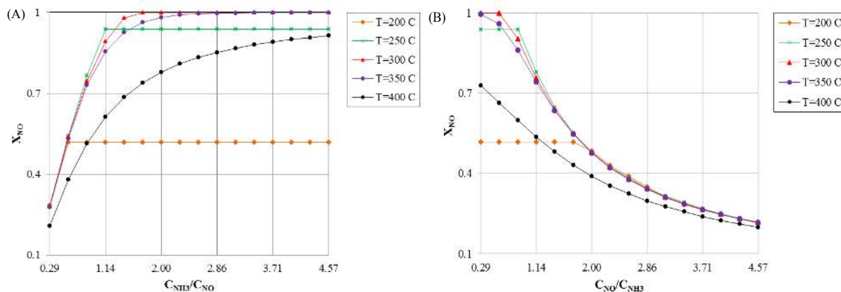
Figure 15: Effect of NO and NH 3 inlet concentrations on NO conversion at different temperatures in the honeycomb reactor, GHSV=5000, (A) C_{NO} =350 ppm, (B) C_{NH_3} =350 ppm, other conditions: see Figure 9.
