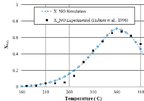
Figure 5: The validation of simulation data with experimental results from catalytic filter candle experiments using ceramic material in a bench-scale test facility ( C_{\text{NO, in}}=C_{\text{NH}_3, in}=350 ppm, C_{\text{O}_2, in}=7.6 vol.%, \text{GHSV}=11000 h -1 , u_{\text{eff}}=0.047-0.073 m/s). Reprinted (adapted) with permission from Nahavandi (2014). Copyright (2014) American Chemical Society.
