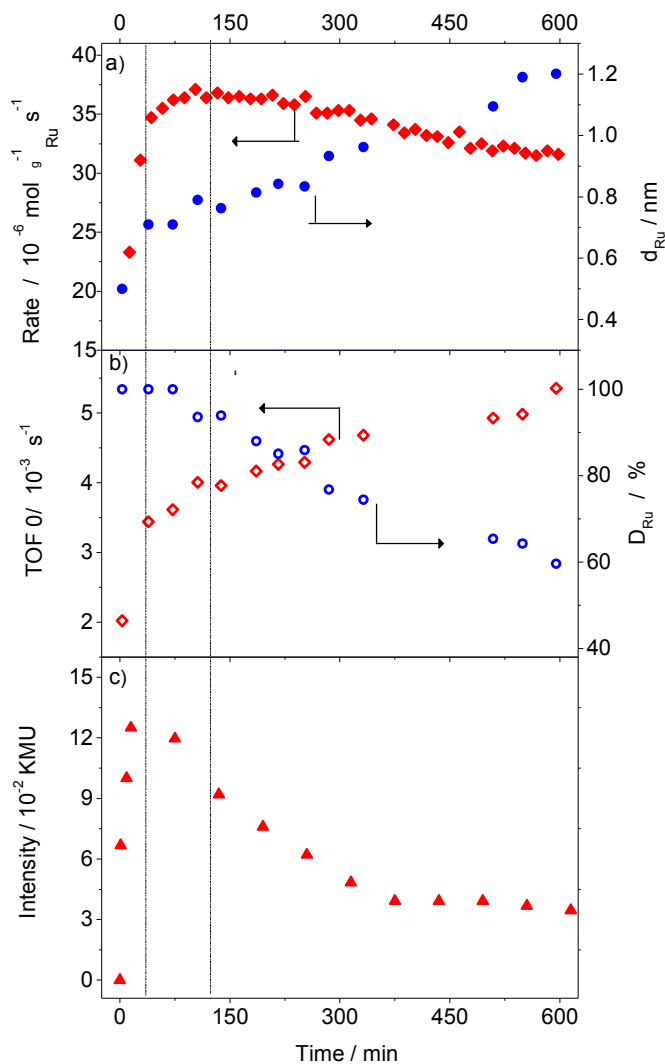
Figure 9 Time evolution of a) the Ru particle size (●), the CO methanation rate (data from Fig. 1b, ◆), b) Ru dispersion (○), turnover frequency (◇), and c) on top \text{CO}_{\text{ad}} intensity (data from Fig. 4b, ▲: band 2009 \text{ cm}^{-1} ) during CO methanation in a ID-ref 6000 gas mixture. The inset in c) shows the evolution of KMU intensity in the first 10 min. Dashed lines indicate the two activation phases and the deactivation phase ( >120 \text{ min} ).
