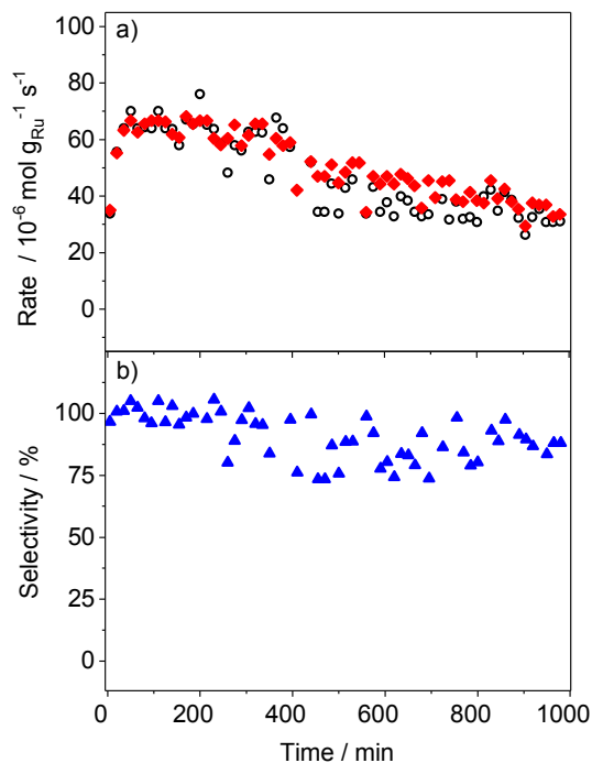
Figure 2 a) Activity ( \blacklozenge : \text{CH}_4 formation; \circ : CO methanation) and b) selectivity ( \blacktriangle ) during the selective CO methanation in SR-ref 100 at 190^\circ\text{C} over the Ru/ \text{TiO}_2 -1 catalyst.
