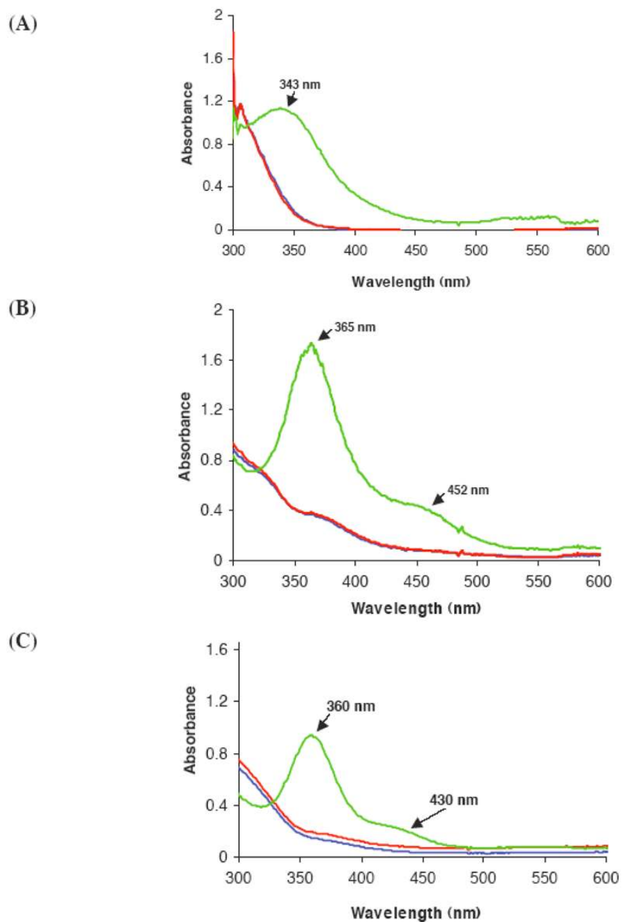
Figure 6. UV-Vis spectra of the reaction of complexes 1 (A), 2 (B) and 3 (C) respectively with excess H 2 O 2 and NEt 3 , (1: 10: 10) recorded at 213 K in CH 3 OH: — 1 mM solution of copper(II) complex; — after addition of 10 mM H 2 O 2 ; — after addition of 10 mM NEt 3
