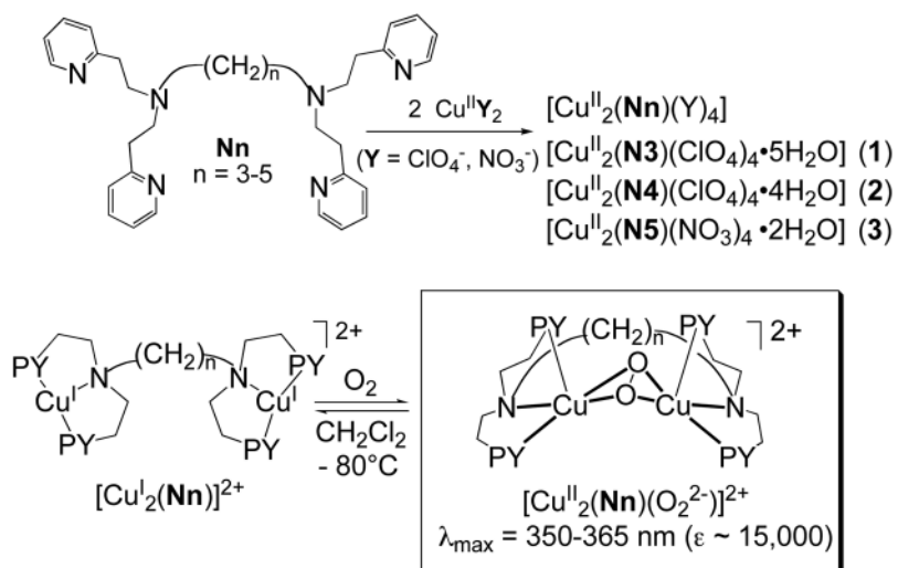
Figure 1. Synthesis of complexes [\text{Cu}^{\text{II}}_2(\text{Nn})(\text{Y})_4] ( \text{Y} = \text{ClO}_4^- or \text{NO}_3^- ) and known dioxygen chemistry of [\text{Cu}^{\text{I}}_2(\text{Nn})(\text{CH}_3\text{CN})_2]^{2+} complexes ( n = 3-5 ).
