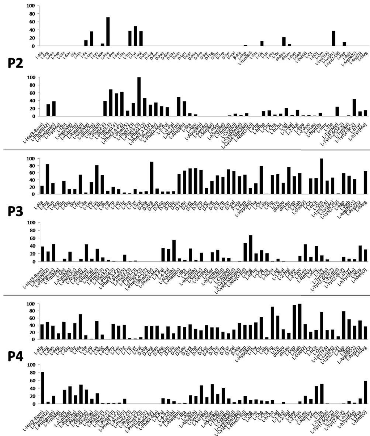
Fig. 2 Human cathepsin L preferences at the P4, P3 and P2 positions. Human cathepsin L preferences were determined using three HyCoSuL sub-libraries, Ac-P4-Mix-Mix-Arg-ACC, Ac-Mix-P3-Mix-Arg-ACC and Ac-Mix-Mix-P2-Arg-ACC, all containing natural and unnatural amino acids. The x axis shows the abbreviated names of the amino acids and the y axis displays the relative activity presented as a percentage of the best-recognized amino acid. Standard deviations calculated from three screenings were 15% of values shown in the figure.
