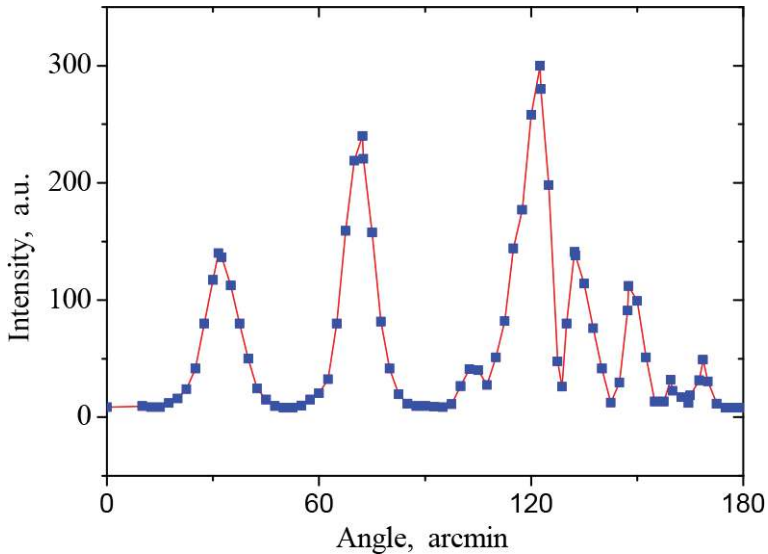
Figure 3. Angular distribution of light beams associated with the set of excited channel modes.
