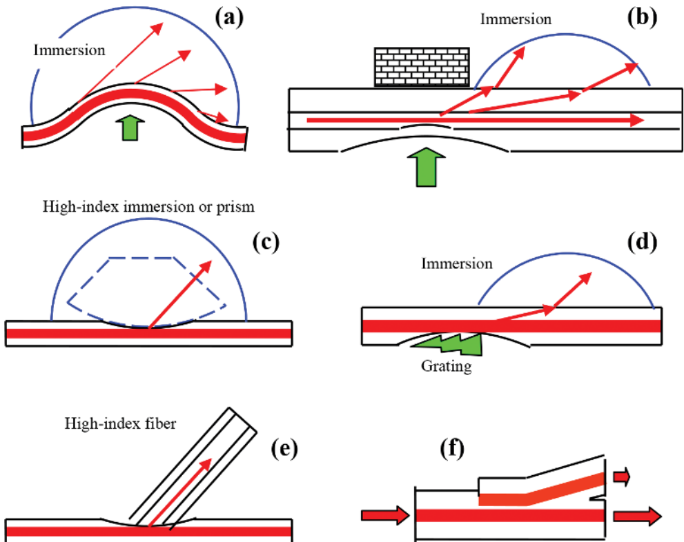
Figure 4. Variants of impact on the fiber resulting in partial extraction of the optical power from the fiber modes: fiber bending (a), local pressing (b), prism-like (c), and diffractive (d) couplers, higher-index fiber (e) and as all-fiber coupler (f).
