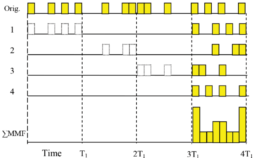
Figure 6. Time distribution of data bit blocks by the modes of the trunk fiber.
