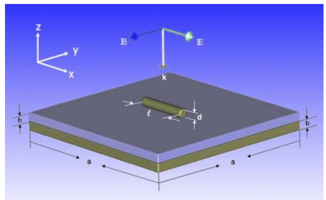
FIG. 1. (Color online) The scheme of plasmonic coupling system: a gold nanorod lay on a gold slab separated by a 10 nm \text{SiO}_2 layer. The structure is surrounded by water. A linearly polarized plane wave illuminated normally onto the slab surface with its electric field along the axis of nanorod.
