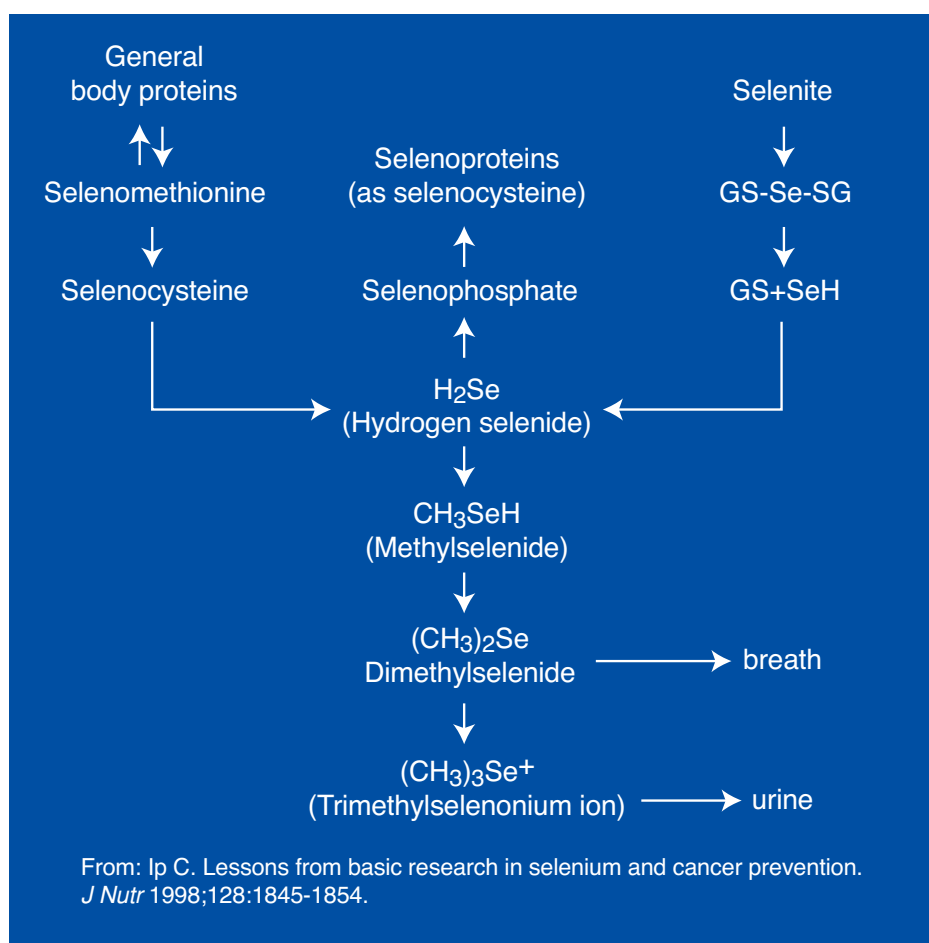
Figure 1. Selenium Metabolism 2
