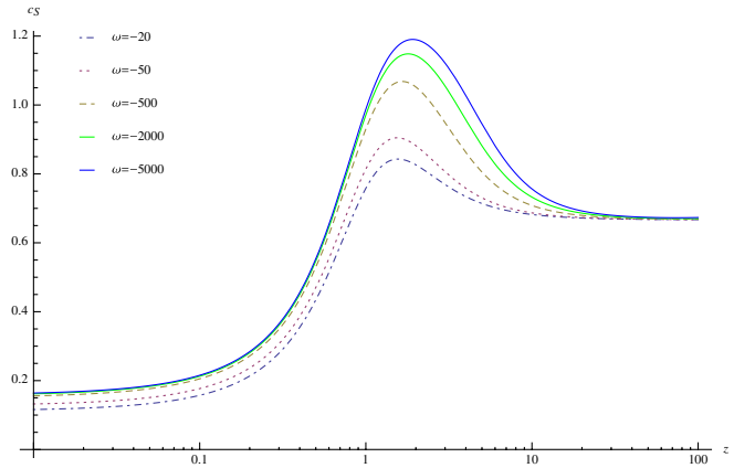
FIG. 3 (color online). Plot of c_s as a function of redshift for various values of the Brans-Dicke parameter. As can be seen during the transition to the accelerating phase the perturbations go superluminal for \omega \lesssim -190 .
