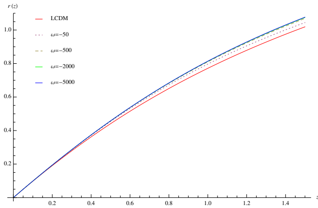
FIG. 2 (color online). The comoving distance r(z) as a function of redshift for different values of \omega .
