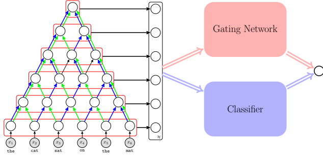
Figure 1: The overall diagram of AdaSent (better viewed in color). Flows with green and blue colors act as special cases for recurrent neural networks and recursive neural networks respectively (see more details in Sec. 3.2). Each level of the pyramid is pooled and the whole pyramid reduces into a hierarchy \mathcal{H} , which is then fed to a gating network and a classifier to form an ensemble.
