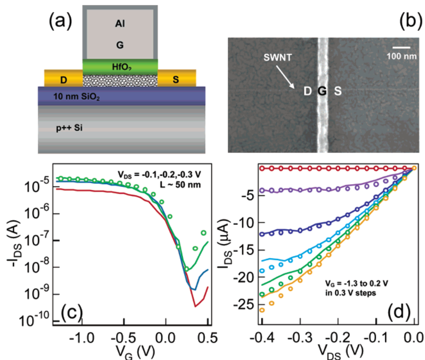
Figure 1. Self-aligned near-ballistic SWNT-FETs. (a) Side-view schematic of a device. SWNTs were grown by chemical vapor deposition 23 on Si(p ++ )/SiO 2 substrates. ALD of HfO 2 used tetrakis(diethylamido)hafnium (Hf[NET 2 ] 4 ) as precursor. For each of the 80 ALD cycles (~0.1 nm/cycle) used, the purge times were 350 s after the DI H 2 O dose, and 150 s after the Hf[NET 2 ] 4 dose. The deposition of Pd was by highly directional electron beam evaporation. For all of our measurements, the bottom gate (Si substrate) was grounded. (b) Scanning electron microscopy (SEM) image showing the top view of a device. The nanotube appears faint under the thin Pd electrodes. (c) Current vs top-gate voltage ( I_{DS}-V_G ) for a device with L \sim 50 nm and d \sim 1.7 nm SWNT at different biases ( V_{DS} ). The devices were annealed in Ar at 175 °C for 5 min to obtain optimum Pd-SWNT contacts. PMMA passivation 24 was used for the measurements. The annealing and passivation treatment steps afforded up to 2–5-fold increase in the p-channel conductance of SWNT FETs. (d) I_{DS}-V_{DS} characteristics of the same device. Solid lines are experimental data and symbols are ballistic quantum simulation in (c) (symbols correspond to V_{DS} = 0.3 V) and (d). Parameters used in simulations (J. Guo et al., to be published): band-gap E_G = 0.5 eV (see Figure 2), SB height for holes \sim 0 , and geometrical parameters identical to experiments.
