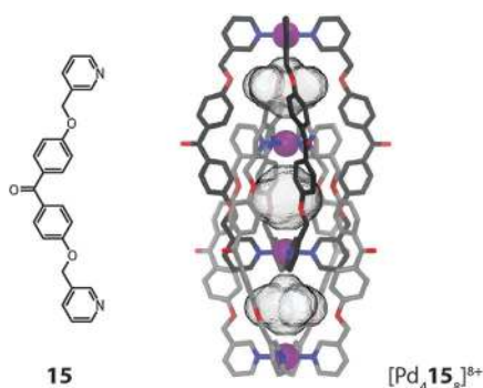
Fig. 13 X-ray structure of the interpenetrated double-cage [Pd_4\mathbf{15}_8]^{8+} .
