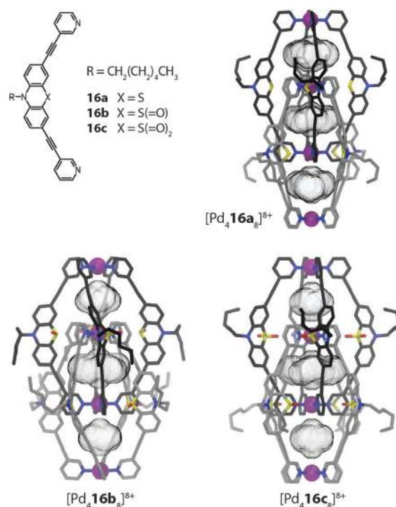
Fig. 14 X-ray structures of three related interpenetrated double-cages [Pd_4\mathbf{16a-c}_8]^{8+} based on phenothiazine and its mono- and di-oxygenated derivatives.
