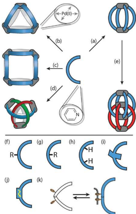
Fig. 1 Overview of discussed [\text{Pd}_n \text{L}_{2n}] ( n = 2-4 ) cages including (a) simple [\text{Pd}_2 \text{L}_4] cages, (b) [\text{Pd}_3 \text{L}_6] and (c) [\text{Pd}_4 \text{L}_8] rings, (d) a [\text{Pd}_3 \text{L}_6] double-trefoil knot with intertwined ligands, and (e) interpenetrating [\text{Pd}_4 \text{L}_8] cage dimers. Ligand functionalisations include substitution in (f) exterior or (g) endo-hedral positions, (h) the placement of hydrogen-bond donors inside the cavity, (i) the introduction of steric bulk around the ligand backbone, and the implementation of (j) redox activity or (k) photo-switchability into the ligand backbones.
