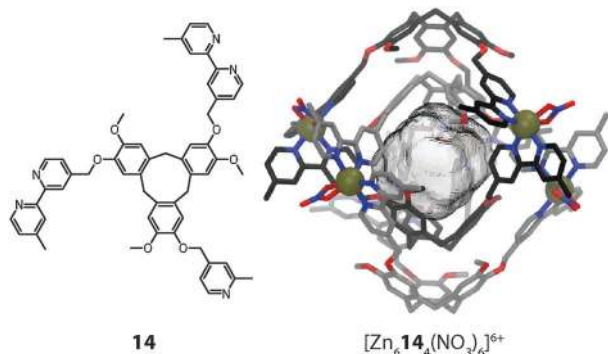
Fig. 12 X-ray structure of the cyclotrimeratrylene-based interpenetrated double-cage [M_6\mathbf{14}_4(NO_3)_6]^{6+} .
