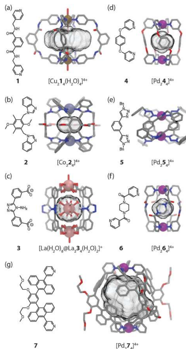
Fig. 2 X-ray structures of cages (a) [\text{Cu}_2 \mathbf{1}_4 (\text{H}_2\text{O})_4]^{4+} , (b) [\text{Co}_2 \mathbf{2}_4]^{4+} , (c) [\text{Ln}(\text{H}_2\text{O})_8]@[\text{Ln}_2 \mathbf{3}_4 (\text{H}_2\text{O})_2]^+ , (d) [\text{Pd}_2 \mathbf{4}_4]^{4+} , (e) [\text{Pd}_2 \mathbf{5}_4]^{4+} , (f) [\text{Pd}_2 \mathbf{6}_4]^{4+} and (g) [\text{Pd}_2 \mathbf{7}_4]^{4+} . For all figures applies: hydrogens, solvent molecules and counter anions were omitted for clarity; C: grey, O: red; N: blue; Cu: brown; Pd: purple; Co: light blue; and La: light red; metal cations are represented as spheres; cavities are depicted as translucent grey potatoids.
