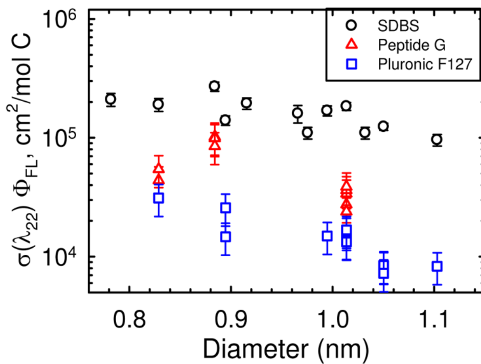
Figure 6. Measured fluorescence action cross sections of selected SWCNT structures suspended in aqueous SDBS (circles), peptide K_2(QL)_5K_2 (G) (triangles), and Pluronic F127 (squares). Data for SWCNTs in SDBS are taken from Ref. 9.
