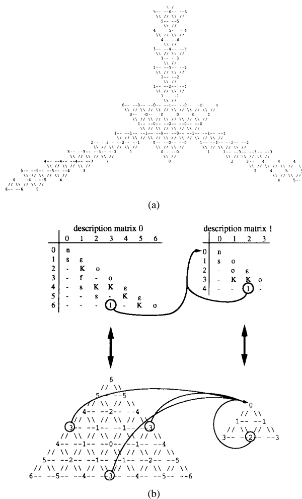
Fig. 17. Construction with two description matrices. An example of (a) iterative structure and (b) description matrices.
