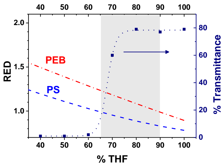
Figure 1. The relative energy difference (RED) of polystyrene (PS, blue dashed line) and poly(ethylene-butylene) (PEB, red dash-dotted line) calculated from Hansen solubility parameters of the polymers and turbidity measurements of the 14 wt% SEBS block copolymer solutions (■) in THF/DMF solvent mixtures (see Table S1, ESI). The navy dotted line shows a Boltzman fit to the turbidity measurements.
