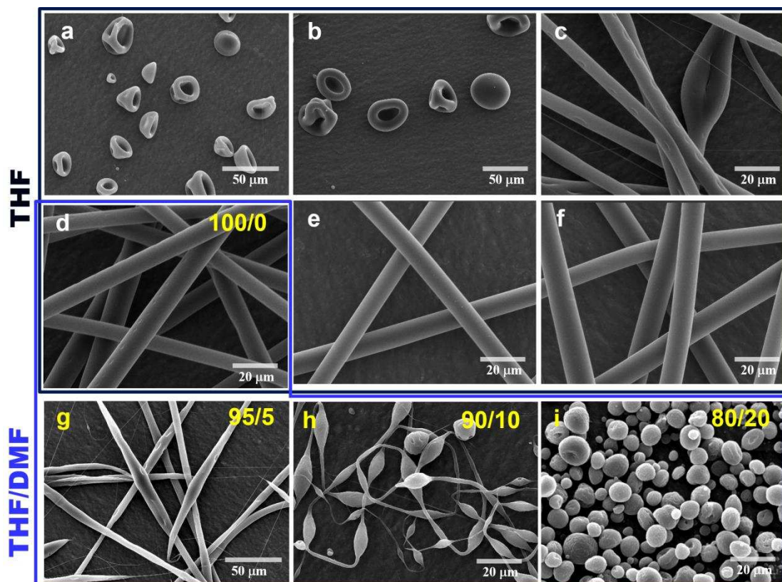
Figure 2. SEM images of electrospun beads (a and b) and electrospun fibers (c – f) of SEBS from neat THF solutions at varying polymer concentrations (8 wt%, 10wt%, 12 wt%, 14wt%, 16 wt% and 18wt% for a - f, respectively). SEM images (d, g-i) show the effect of
