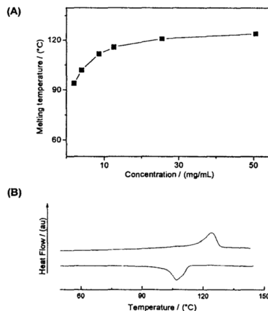
Figure 1. A) Variation of the melting temperature a gel of 2 in tetralin with the concentration of 2 . B) DSC heating (top) and cooling (bottom) traces of a gel of 2 in tetralin (10 mg mL -1 ).
