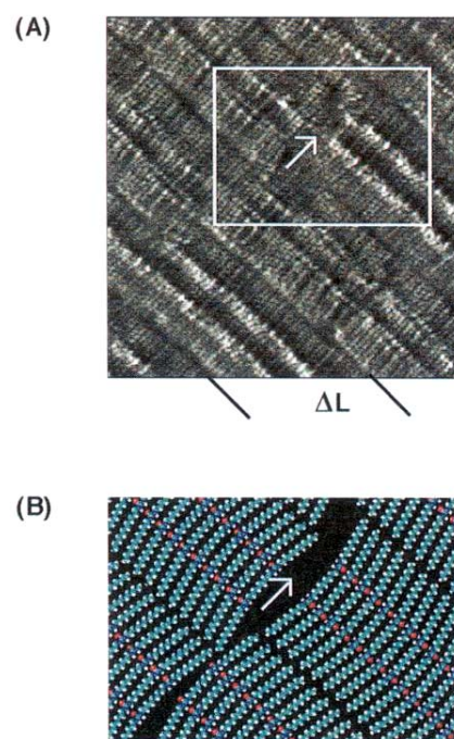
Figure 3. A) STM image of an ordered monolayer of 2 formed by physisorption from 1-octanol at a liquid/graphite interface. Image size: 13.5 \times 13.5 nm 2 , \Delta L is the width of one ribbon of molecules of 2 . The arrow indicates the defect where hydrogen bonds are broken. B) Molecular model for the two-dimensional packing of 2 .
