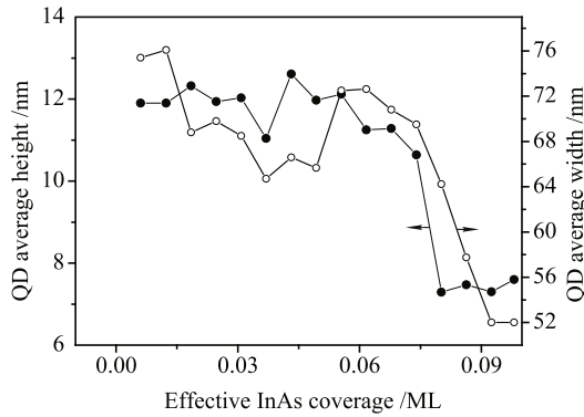
Fig. 6 Average height and width of QDs, h_{ave} and w_{ave} , vs. the effective InAs coverage for F = 1.0 ML/s.
