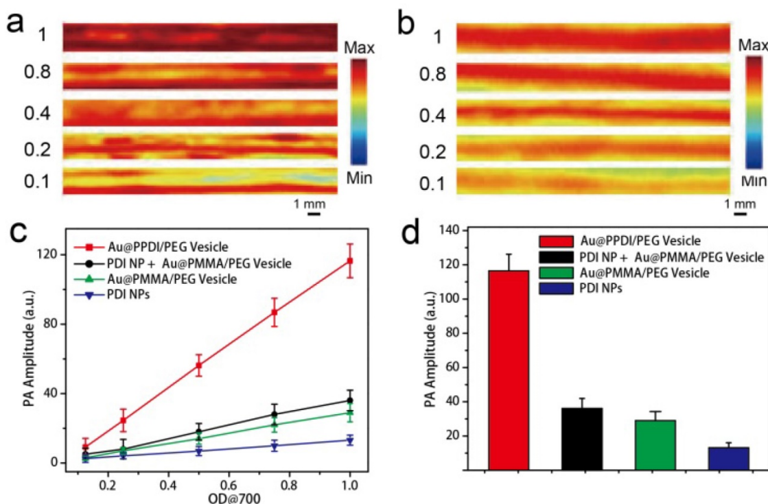
Figure 3. PA images of (a) Au@PPDI/PEG vesicle and (b) the mixture of Au@PMMA/PEG vesicles and PDI NPs aqueous solutions, (c) PA amplitudes of the samples in aqueous solution as a function of OD 700 value. (d) PA amplitudes of the samples at the OD 700 value is 1.0.
