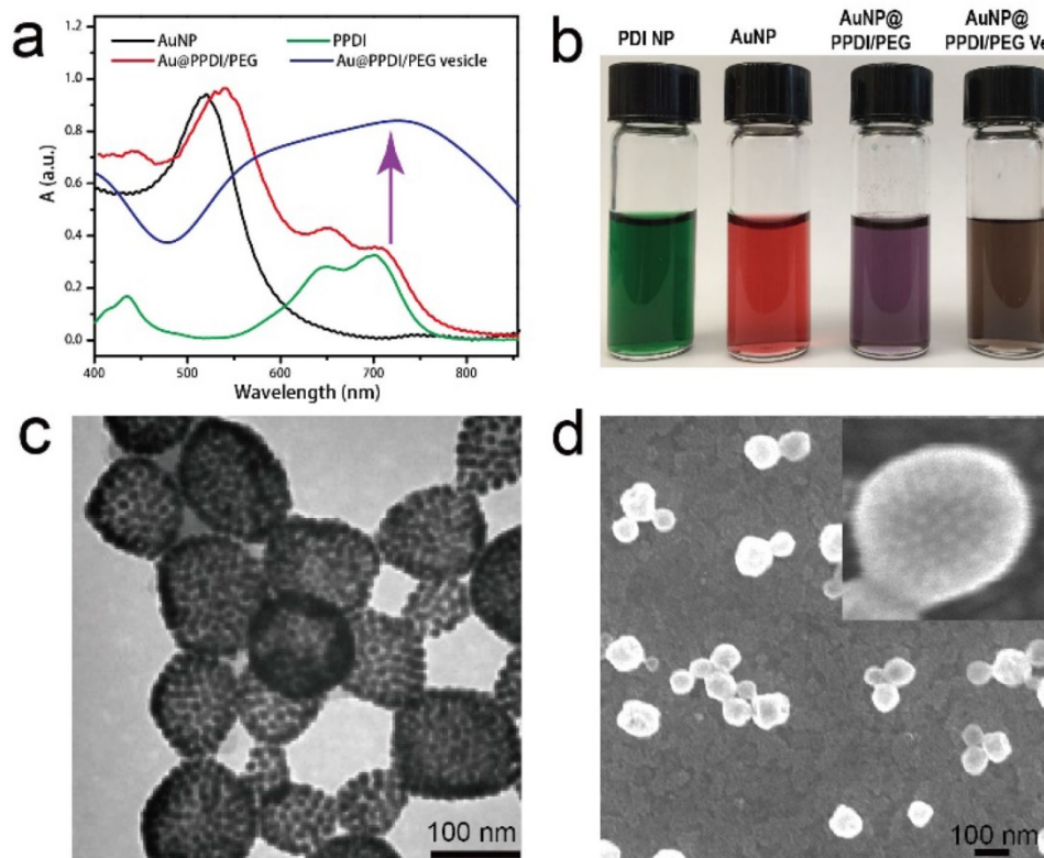
Figure 2. (a) UV-vis spectra of the Au NPs in water, PDI and Au@PPDI/PEG in chloroform, and the Au@PPDI/PEG vesicles in water. (b) Photographs of the samples in water. TEM (c) and SEM (d) images of Au@PPDI/PEG vesicles.
