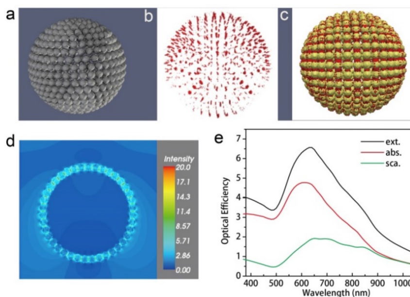
Figure 5. Optical efficiency and near-field distribution of the vesicle calculated using the discrete dipole approximation. A 3D model of the vesicle (a), representation of the hot spots (red) (b) and overlaid image (c) with local field enhancement of a factor of five or larger at the incident wavelength of 700 nm. The Au nanospheres are shown in yellow. (d) Near-field distribution in a x-y cross-section close to the center of the vesicle at the incident wavelength of 700 nm. Only electric field strength is shown. (e) The optical efficiency of the vesicle shown in its extinction (black), absorption (red), and scattering (blue) spectra.
