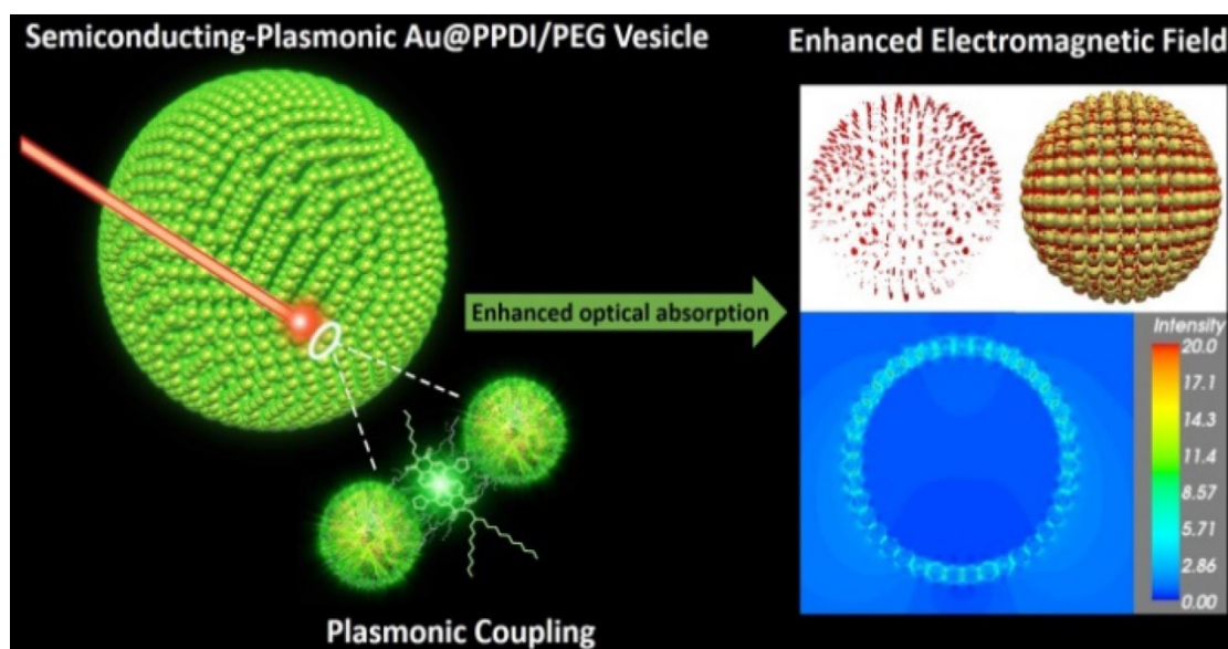
Figure 1. Schematic illustration of the semiconducting-plasmonic vesicle of gold nanoparticle coated with PPDI and PEG. The strong electromagnetic field in the vesicular shell is due to interparticle plasmonic coupling, leading to enhanced optical property.
