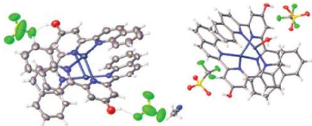
Fig. 3 Solid-state molecular structures of 2 and 2-a (respectively) demonstrating the bridging-helical arrangement of the ligand system.
