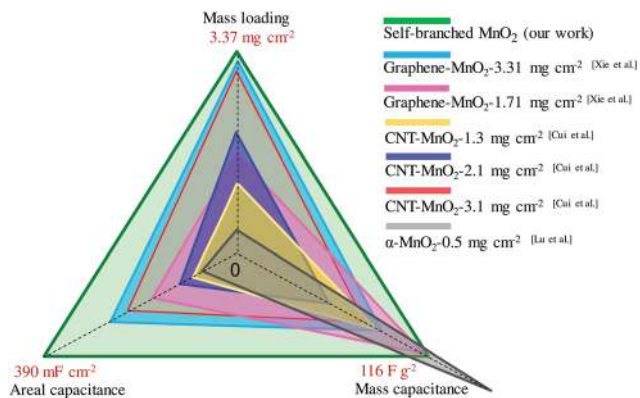
Fig. 6 Capacitance comparison with previous studies considering mass loading. All the capacitance values were obtained at a scan rate of 20 \text{ mV s}^{-1} .
