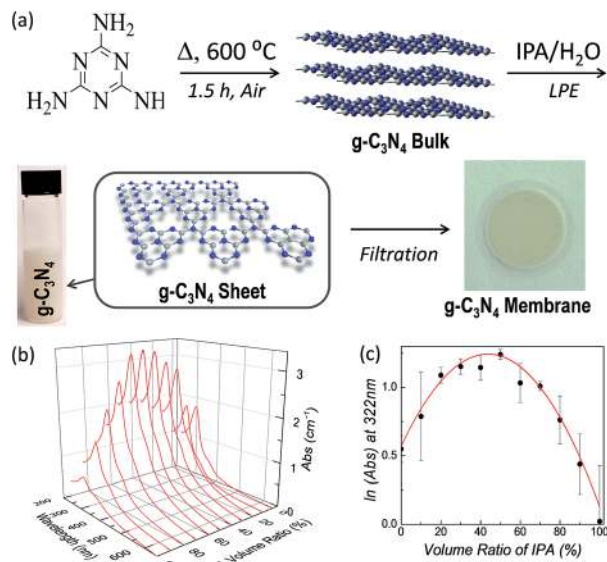
Fig. 1 (a) Schematic of the synthesis of g\text{-C}_3\text{N}_4 bulk and its liquid phase exfoliation in mixed solvents: the bulk graphitic carbon nitride is prepared by thermal annealing of melamine, followed by liquid-phase exfoliation in IPA/water. Membranes are obtained by using vacuum filtration. (b) Typical UV-Vis spectra of dispersed g\text{-C}_3\text{N}_4 in IPA/ \text{H}_2\text{O} mixtures (diluted 10 times). (c) Concentration of dispersed g\text{-C}_3\text{N}_4 as a function of the solvent ratio. The red line is the fit obtained by using eqn (1) (see main text).
