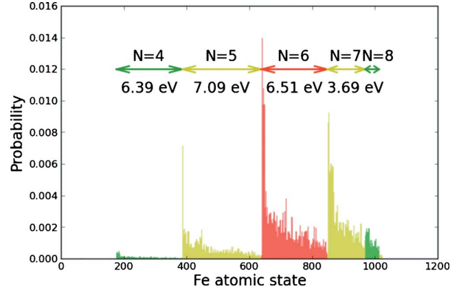
FIG. 4. (Color online) The atomic histogram of the Fe- 3d shell for \text{BaFe}_2\text{As}_2 . The atomic states (all 1024) are sorted according to their valence N . Below the arrow we also display the multiplet splitting of the atomic states in each valence. The N=5 and N=6 valences show the largest splitting of 7 and 6.5 eV, resulting in a very broad lower Hubbard band of the one electron density of states.
