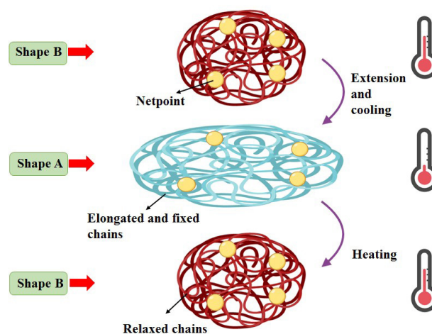
Fig. 1. Shape memory effect in polymers.
