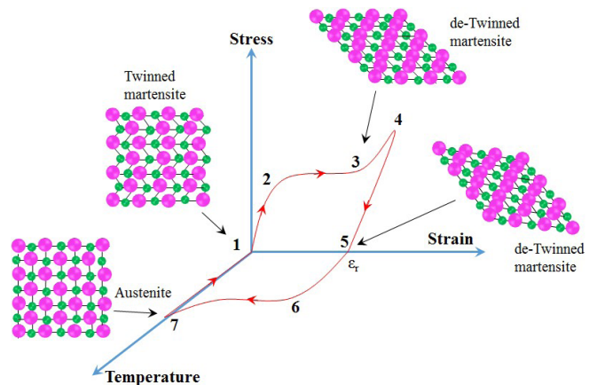
Fig. 3. Shape memory effect in SMAs.
