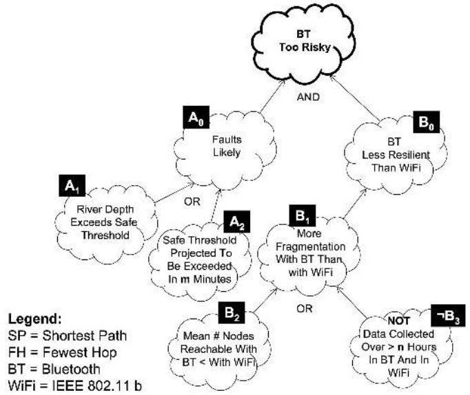
Figure 5. GridStix Claim Refinement Model Justifying Choice of WiFi for Inter-Node Communication
