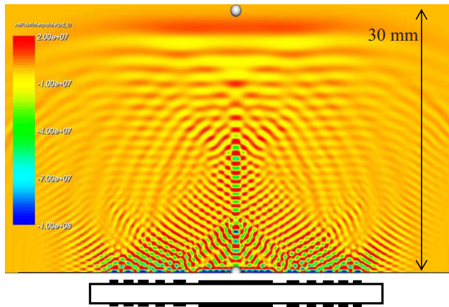
FIG. 1. (Color online) The simulated wave pressure distribution generated by a FZP in glycerin at t=7.009\ 35\ \mu\text{s} (Ref. 19).
