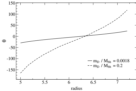
Figure 1. Stable equilibria for a disk of constant surface density.
