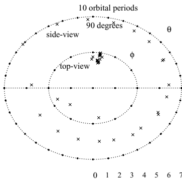
Figure 2. Time evolution of a disk with mass M_d = 0.25M_{bh} . After 10 orbital periods the disk dissolves into subrings, hence is unstable.
