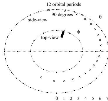
Figure 3. As in figure 2, but for a disk having M_d = 0.05M_{bh} . The rings still lie on the same LONs after 12 orbital periods, hence the disk is stable.
