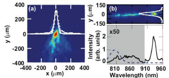
FIG. 2: (color)(a) The laser spot at the exit of the gas cell. (b) Spectrally- and spatially-resolved (in \hat{y} ) laser spot at the exit of the gas cell. Note that the spectrum up to 900 \text{ nm} has been suppressed by 50\times to compensate for the falling quantum efficiency of the CCD camera at longer wavelengths. The original laser spectrum (dashed line) is also shown.
