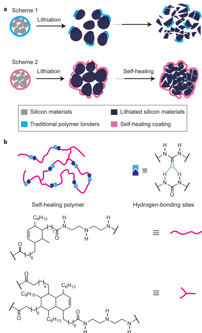
Figure 1 | Design and structure of the self-healing electrode. a , Scheme 1: schematic illustration of the design and behaviour of a conventional silicon electrode that shows failure of the electrode because of cracking in particles and polymer binder, which results in loss of electrical contact. Scheme 2: schematic illustration of the design and behaviour of our stretchable self-healing electrode that shows the maintaining of electrical contact between the broken particles and no cracks in the polymer binder because of the stretchability and incorporation of self-healing chemistry. b , Chemical structure of the SHP. Magenta lines, polymer backbones; light-blue and dark-blue boxes, hydrogen-bonding sites.
