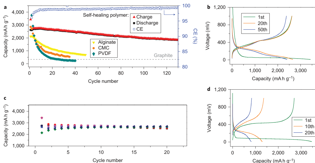
Figure 3 | Electrochemical properties of SiMP electrodes. a , Capacity retention of SiMP electrodes with different polymer additives, including the SHP/CB composite and conventional polymer binders (PVDF, CMC and alginate). All samples were cycled at the same charge/discharge rate of C/10 with a potential window of 0.01–1 V versus \text{Li}/\text{Li}^+ . The grey dashed line indicates the theoretical capacity of a graphite electrode. The SiMP electrode with SHP showed a much longer cycling lifetime than that of conventional polymer binders. b , Voltage profiles of a SiMP/SHP/CB electrode at the first, 20th and 50th cycles, showing very little capacity decay during the cycling. c , Discharge capacity retention for six different SiMP/CMC electrode samples at a charging/discharging rate of C/10 . All six different batches showed similar cycling performance. All the specific capacities are reported based on the weight of the SiMPs. d , Voltage profiles of a SiMP/CMC electrode at the first, 10th and 20th cycles show a much faster capacity decay than that of the self-healing electrode.
