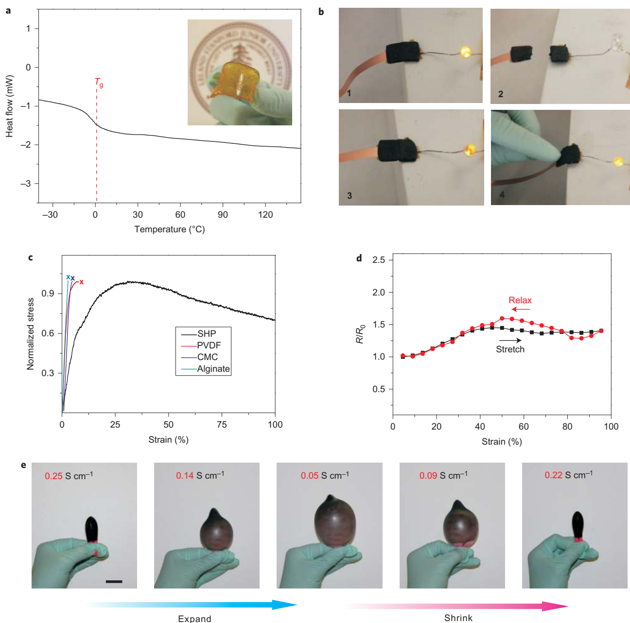
Figure 2 | Characterization of the self-healing composite material. a , DSC curve of the SHP showing that the T_g of SHP is 0\text{ }^\circ\text{C} , much lower than room temperature. Inset: photograph of the SHP. b , Demonstration of the electrical and mechanical self-healing capability of the conductive composite using a battery-powered circuit with the composite SHP as the conductive pathway that connects the LED to the battery. c , Tensile tests of the SHP and other conventional polymer binders show that SHP exhibits much higher stretchability than conventional polymer binders. d , The ratio between the resistance ( R ) and initial resistance ( R_0 ) at different strains shows that the SHP/CB composite remains conductive over the whole stretching cycle. e , The SHP/CB composite material was coated onto an inflatable balloon to mimic the volumetric changes of silicon particles over the cycling process. The changes in its electrical conductivity during the balloon's repeated cycles of inflation and deflation were monitored. The SHP/CB coating remains conductive over the whole expand/shrink process. Scale bar, 2 cm.
