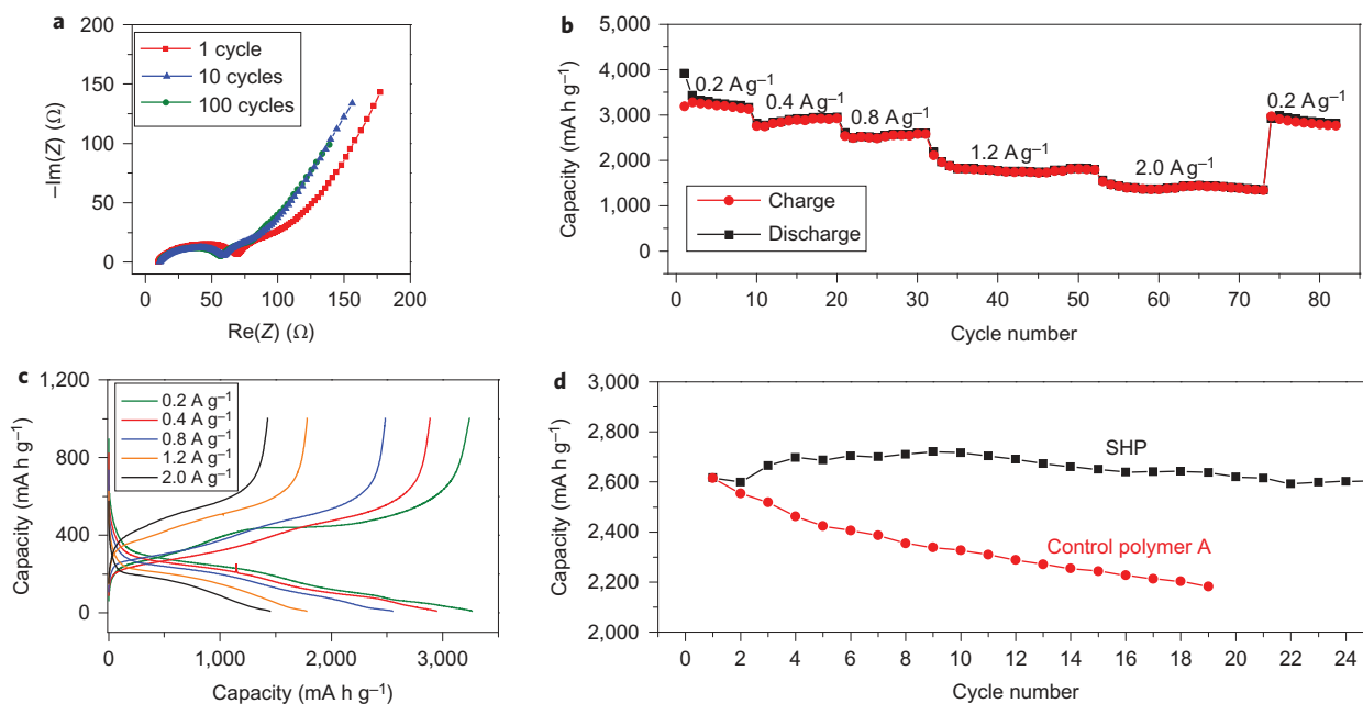
Figure 4 | Cycling properties of the self-healing SiMP electrode. a , Impedance spectroscopy measurements for a SiMP/SHP/CB electrode after different numbers of cycles, showing that no observable impedance increase even after 100 cycles. The real and imaginary parts of the complex impedance Z are denoted by \text{Re}(Z) and \text{Im}(Z) , respectively. b,c , Capacity retention ( b ) and galvanostatic charge/discharge profiles ( c ) of a SiMP/SHP/CB electrode cycled at various current densities, showing the stable cycling stability at different charging/discharging rates. d , Discharge capacity retention of the SiMP electrode with SHP and control polymer A. Control polymer A showed much worse cycling stability than SHP. All samples were charged/discharged at a rate of C/10 . All the specific capacities are reported based on the weight of the SiMPs.
