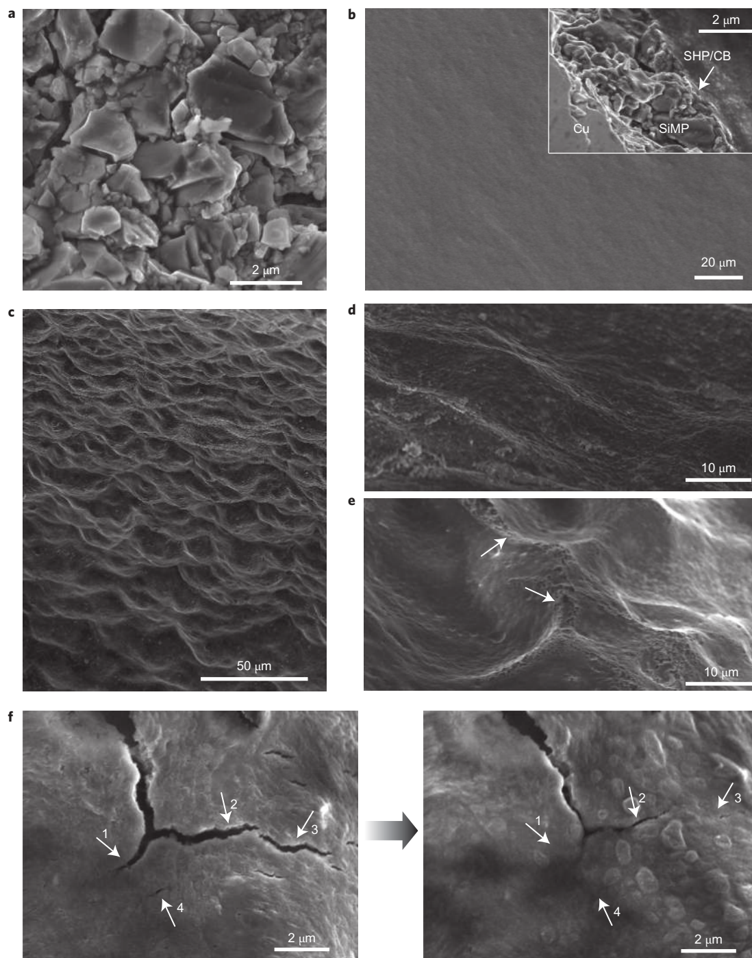
Figure 5 | Structure of the self-healing SiMP electrode during electrochemical cycling. a , Bare SiMPs have a large size distribution. The initial SiMPs have an average diameter of 4.2 \mu\text{m} , with a size-distribution range from 2 to 7 \mu\text{m} . b , Surface morphology of the electrode before cycling. Inset: cross-sectional SEM image of the electrode showing the layered structure. From left to right the layers are (1) a copper layer as the current collector, (2) the SiMP layer as the active material and (3) the self-healing conductive composite (SHP/CB) coating. c , A continuous wave-like morphology of the surface of the electrode is evident after 20 cycles at a rate of C/10 . d , Magnified image of the wave-like structure. e , Some scar-like structures (arrows) can be found on the electrode after the cycling process, which appear to be cracks that subsequently healed. f , Left: cracks in the polymer layer in the lithiated state; right: after five hours the smaller cracks were healed, indicated by the arrows on the images.
