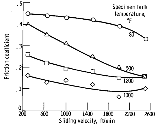
Figure 6. - Friction properties of 40-volume-percent-fluoride and 60-volume-percent-nickel composite bearing materials. Bearing surface of composite coated with 0.002-inch sintered eutectic.
