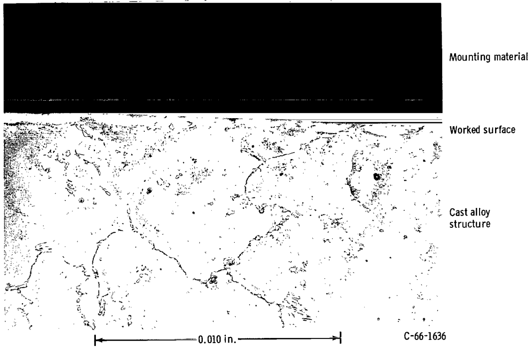
Figure 10. - Section through wear surface of rider specimen run against wear track shown in figure 9.
