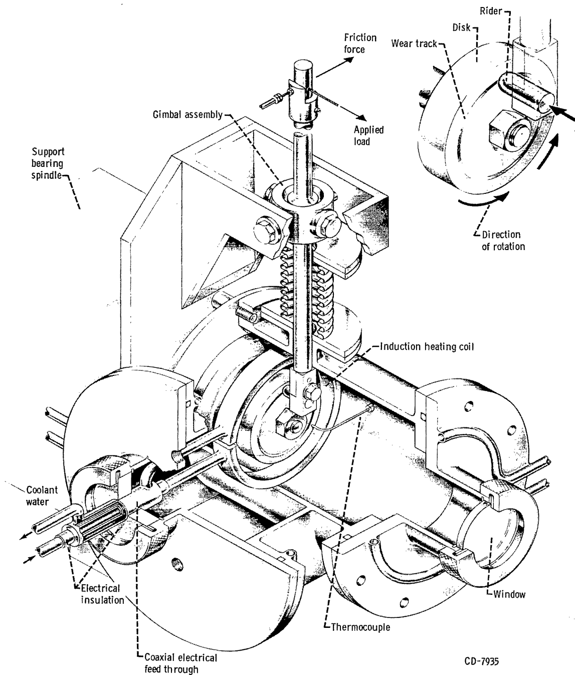
Figure 1. - High-temperature friction apparatus.
