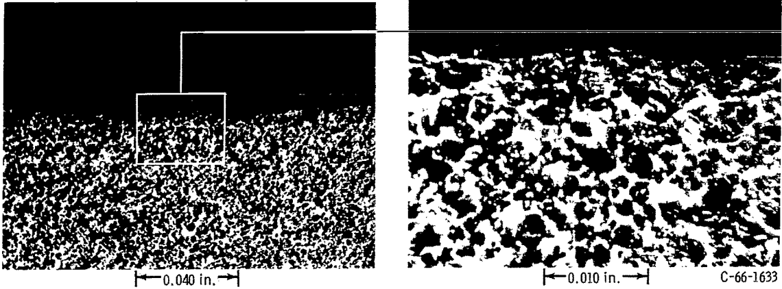
Figure 4. - Section through wear track of 40-volume-percent-fluoride and 60-volume-percent-nickel composite showing mild surface damage caused by 7/8-inch-radius hemispherical rider. Load, 500 grams; rider material, cast nickel-chromium alloy; temperature, 1000° F; sliding velocity, 2000 feet per minute; duration, 1 hour.
