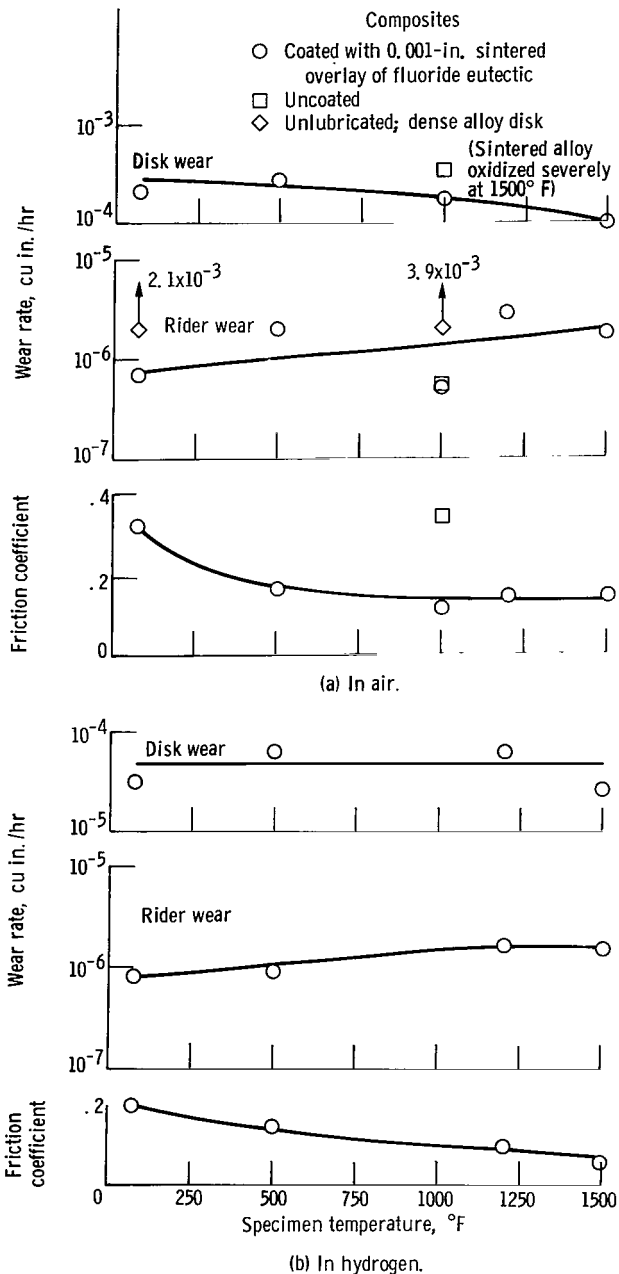
Figure 8. - Lubricating properties of eutectic fluoride and nickel-chromium alloy composites. 35 Volume percent barium fluoride - calcium fluoride eutectic and 65 volume percent sintered alloy; sliding velocity, 2000 feet per minute; load, 500 grams; specimens, nickel-chromium cast alloy riders (7/8-in. hemispherical radius) against composite disks.
