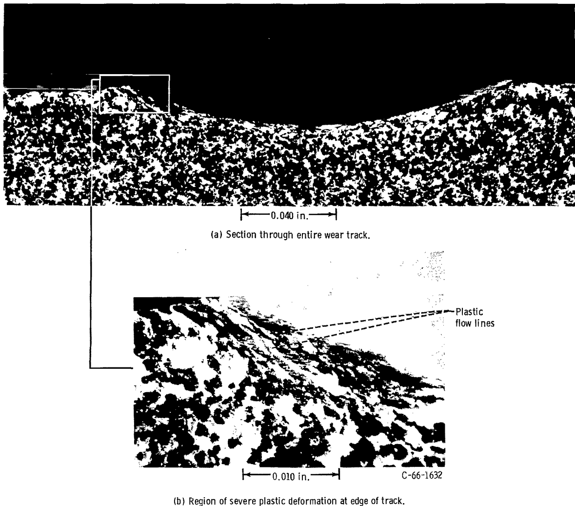
Figure 3. - Sections through wear track of 50-volume-percent-fluoride and 50-volume-percent-nickel composite showing plastic deformation caused by 3/16-inch-radius hemispherical rider. Load, 500 grams; rider material, cobalt-bonded tungsten carbide; temperature, 1000° F; sliding velocity, 2000 feet per minute; duration, 1 hour.
