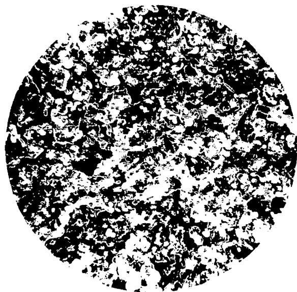
Figure 7. - Photomicrograph of fluoride plus sintered nickel-chromium alloy composite material. 35 Volume percent barium fluoride - calcium fluoride eutectic and 65 volume percent sintered nickel chromium alloy. Prepared by electropolishing and dark field illumination. White areas, fluoride; black areas, metal.
