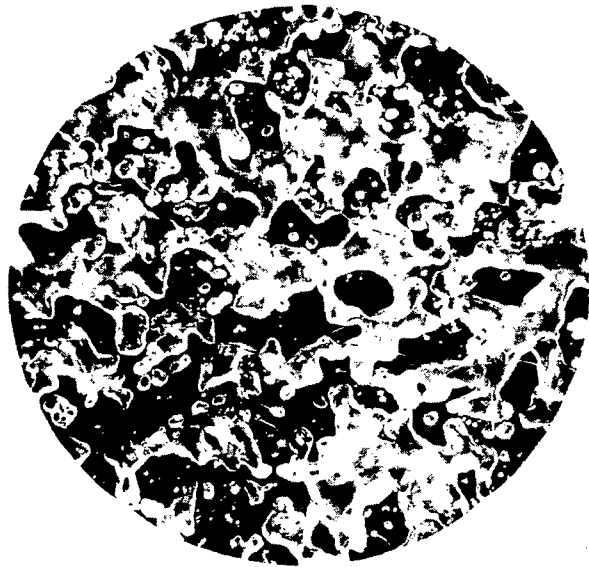
Figure 2. - Photomicrograph of fluoride plus nickel composite material. 50 Volume percent barium fluoride - calcium fluoride eutectic and 50 volume percent nickel. Prepared by electropolishing and dark field illumination. White areas, fluoride; black areas, nickel.
