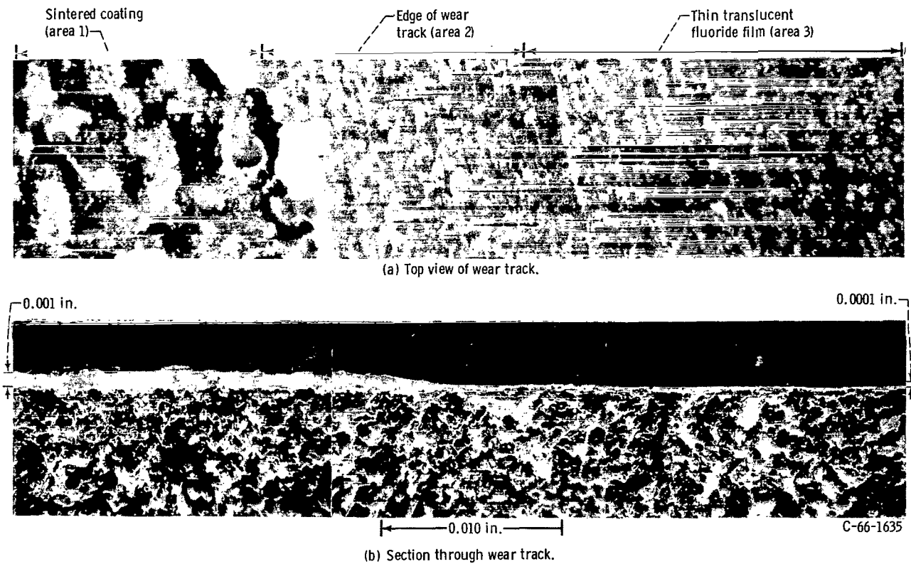
Figure 9. - Montage of wear track on 35 volume percent fluoride plus 65 volume percent alloy composite. Load, 500 grams; temperature, 1200° F (hydrogen); sliding velocity, 2000 feet per minute; duration, 6 hours; rider, 7/8-inch-radius hemisphere.
