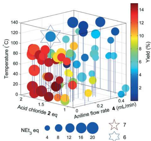
Fig. 4 Multi-dimensional plot, showing the results of the optimization of enolate 7 . The 3-axis plot show the aniline 4 flow rate (x-axis), acid chloride 2 eq. (y-axis) and temperature (z-axis). The size of the point represents \text{NEt}_3 eq., and the colour represents the product yield. The optimum conditions: 0.1 \text{ mL min}^{-1} 4 , 117.8 \text{ }^\circ\text{C} , 1.5 \text{ eq. 2} , 15.2 \text{ eq. NEt}_3 and 12.7 \text{ min} are highlighted by the 5-pointed star. The optimum conditions of 6 are highlighted by the 6-pointed star.
