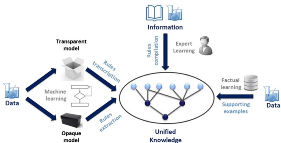
Figure 5 Combining different source of knowledge. Different sources of knowledge can be merged into a structured and unified model. This permits to combine different learning techniques (expert learning, machine learning and facts).
