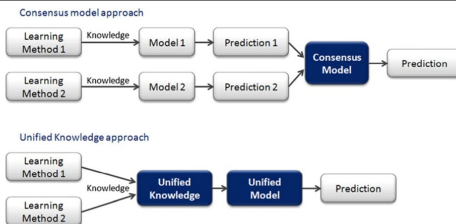
Figure 2 Consensus model vs. Unified knowledge. Two ways of combining different learning methods; the consensus approach by merging the prediction (late stage) and the unified knowledge approach by combining the knowledge (early stage).
