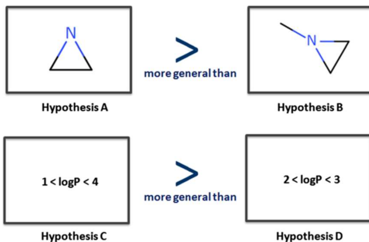
Figure 6 Ordering hypotheses according to their degree of generalisation. Hypotheses can be ordered according to their level of generalisation. Here, hypotheses A is more general than hypothesis B (A is a substructure of B). Similarly C is more general than D.
