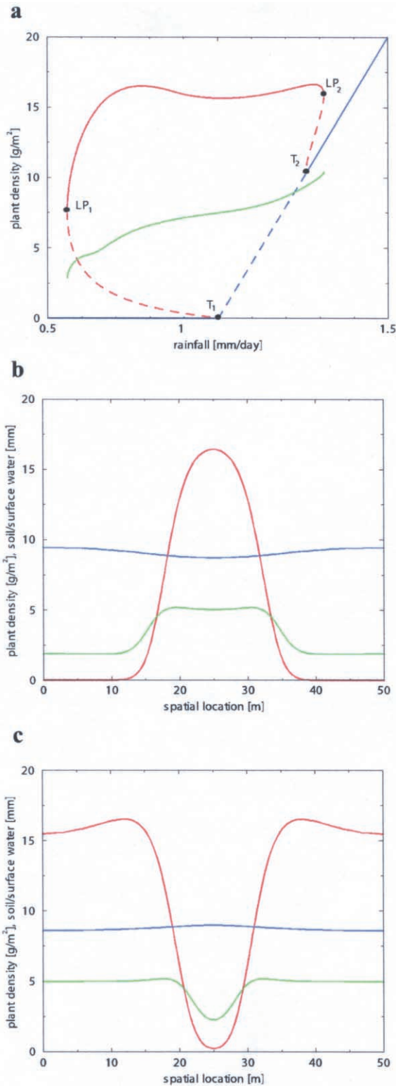
Figure 3: a, Bifurcation diagram based on a one-dimensional model for a spatial range of 50 m. Plant mortality, d , is 0.25, with other parameters as defaults (see text). Spatially homogeneous equilibria are in blue, non-homogeneous equilibria are in red (showing maximum local plant densities). Solid lines denote stable equilibria, whereas dotted lines are unstable equilibria. The green line depicts the average plant density in the stable nonhomogeneous equilibrium. T_1 ( R = 1.001 ) and T_2 ( R = 1.259 ) are Turing instability points, and LP_1 ( R = 0.557 ) and LP_2 ( R = 1.312 ) are limit points. b, Profile of stable plant peak at R = 0.75 . Plant density in red, surface water in blue, and soil water in green. c, Profile of stable plant gap at R = 1.25 ; lines as for b.
