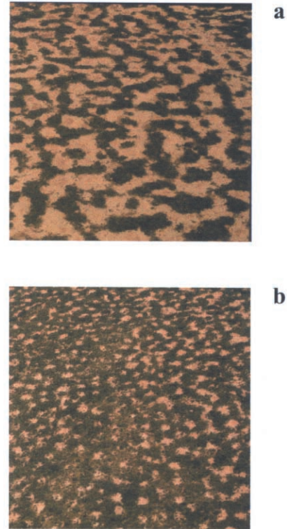
Figure 1: Aerial photographs from patterned vegetation in Niger (S. Prince, personal communication). Scale is 400 \times 400 m. a , Labyrinths with spots; b , gap pattern.
