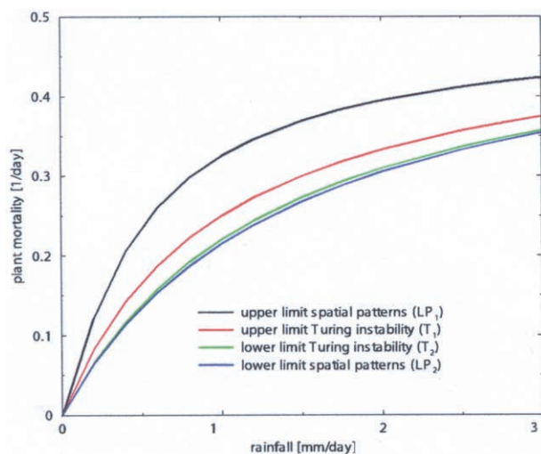
Figure 4: Region of spatial patterns as a function of rainfall and plant mortality. The points LP_1 , T_1 , T_2 and LP_2 from figure 3a are plotted as a function of R and d . Between LP_1 and LP_2 , spatial pattern formation is possible, whereas between T_1 and T_2 , the homogeneous equilibrium is unstable.
