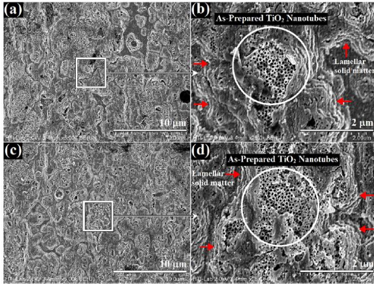
Fig. 1. FESEM top view images of as-prepared \text{TiO}_2 nanotubes in different anodization electrolytes, (a,b) EG and (c,d) G.
