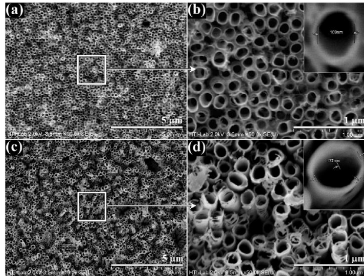
Fig. 3. Microstructural evolutions of the anodized samples after thermal annealing at 600 °C for 2 h, (a,b) EG and (c,d) G.
