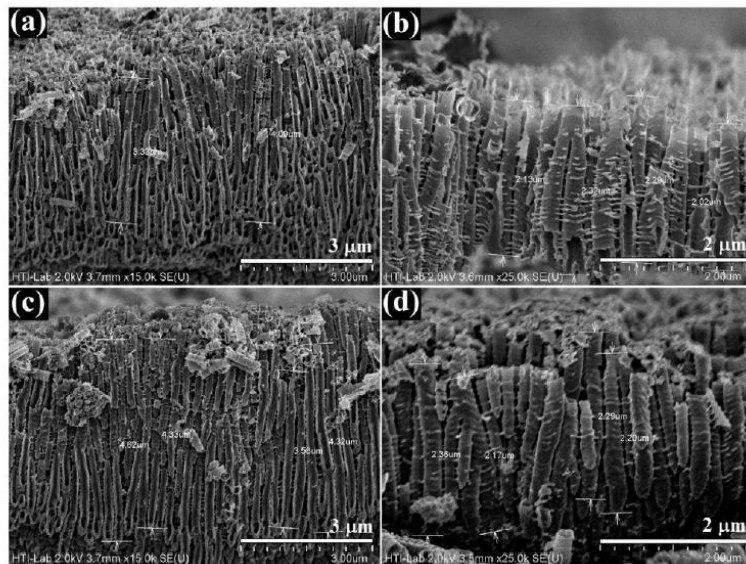
Fig. 4. FESEM cross-section images of TiO 2 nanotubes after 2 h annealing through two electrolytes, (a) EG and (b) G at 450 °C and (c) EG and (d) G at 600 °C.
