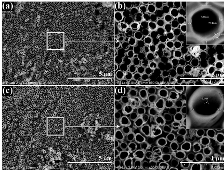
Fig. 2. Microstructural evolutions of the anodized samples after thermal annealing at 450^\circ\text{C} for 2 h, (a,b) EG and (c,d) G.
