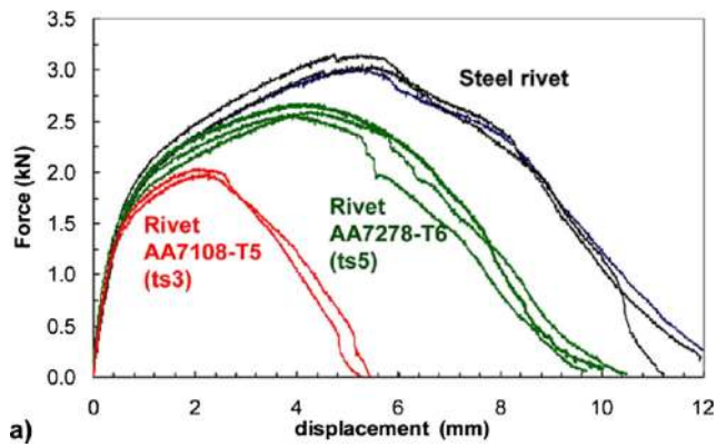
Fig. 7 Comparison of the single-joint strength between aluminium rivets and a steel rivet with combined shearing and pull-out loading with loading angle \alpha = 45^\circ [53]
